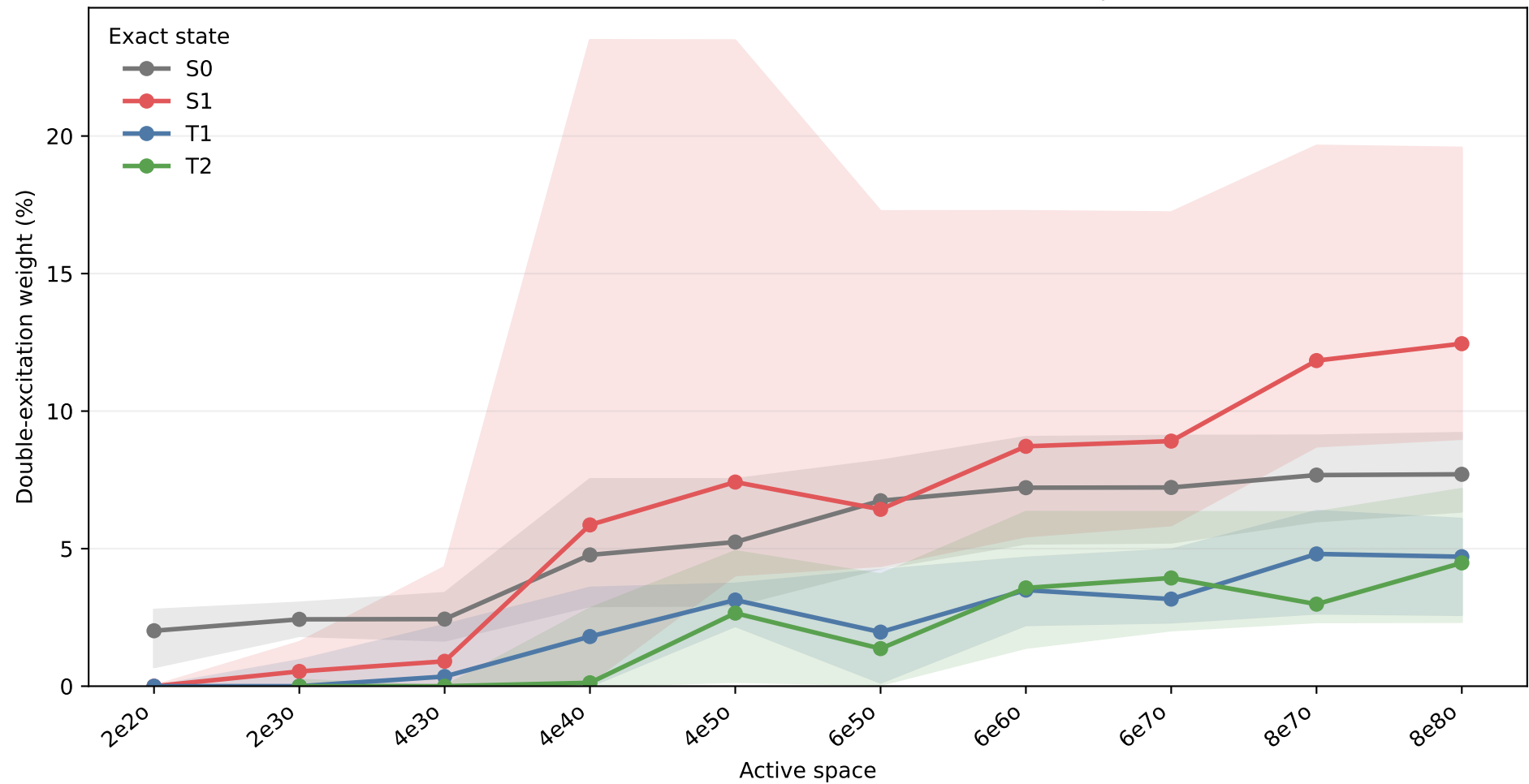
CASCI double-excitation character across active space
