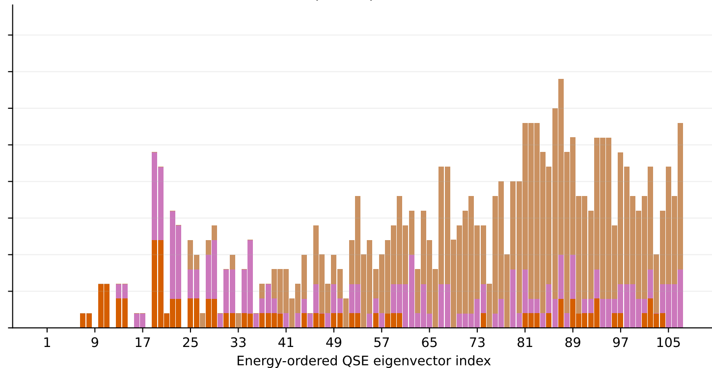
Triplet expansion
