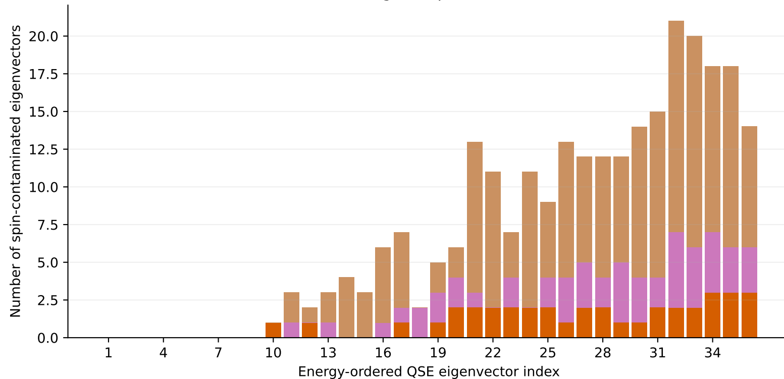
Singlet expansion
