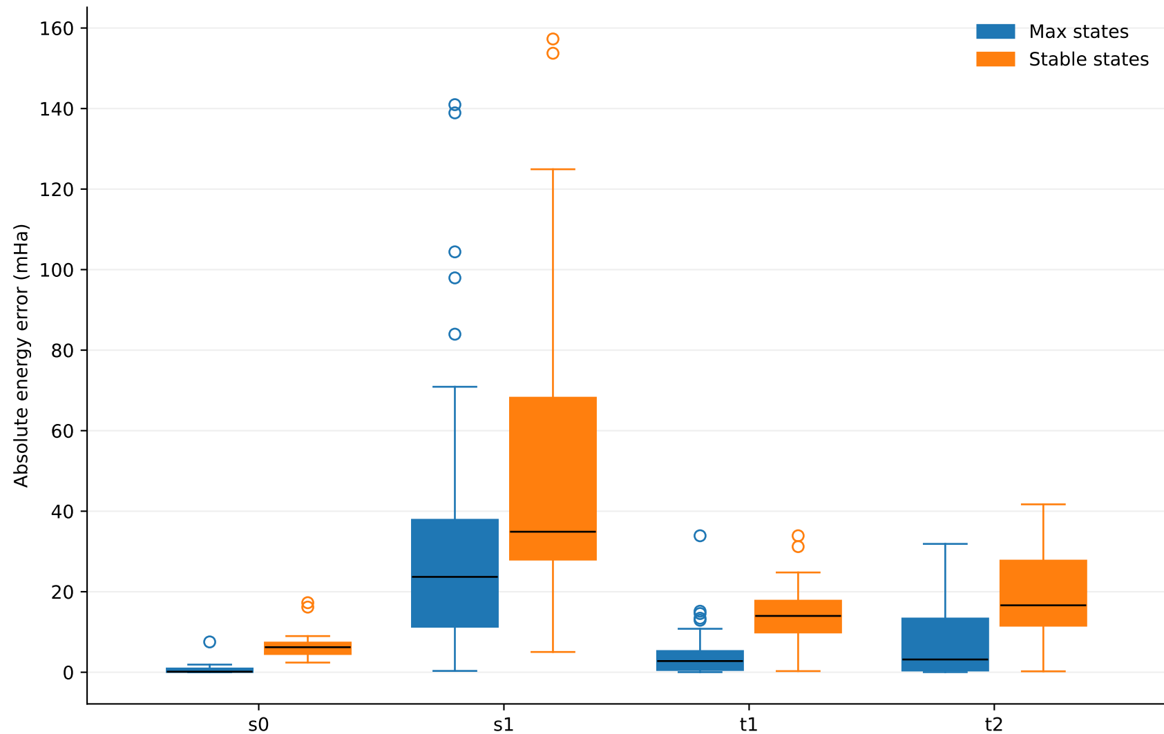
UCCSD 6e6o: Maximum and Stable QSE Dimensions
