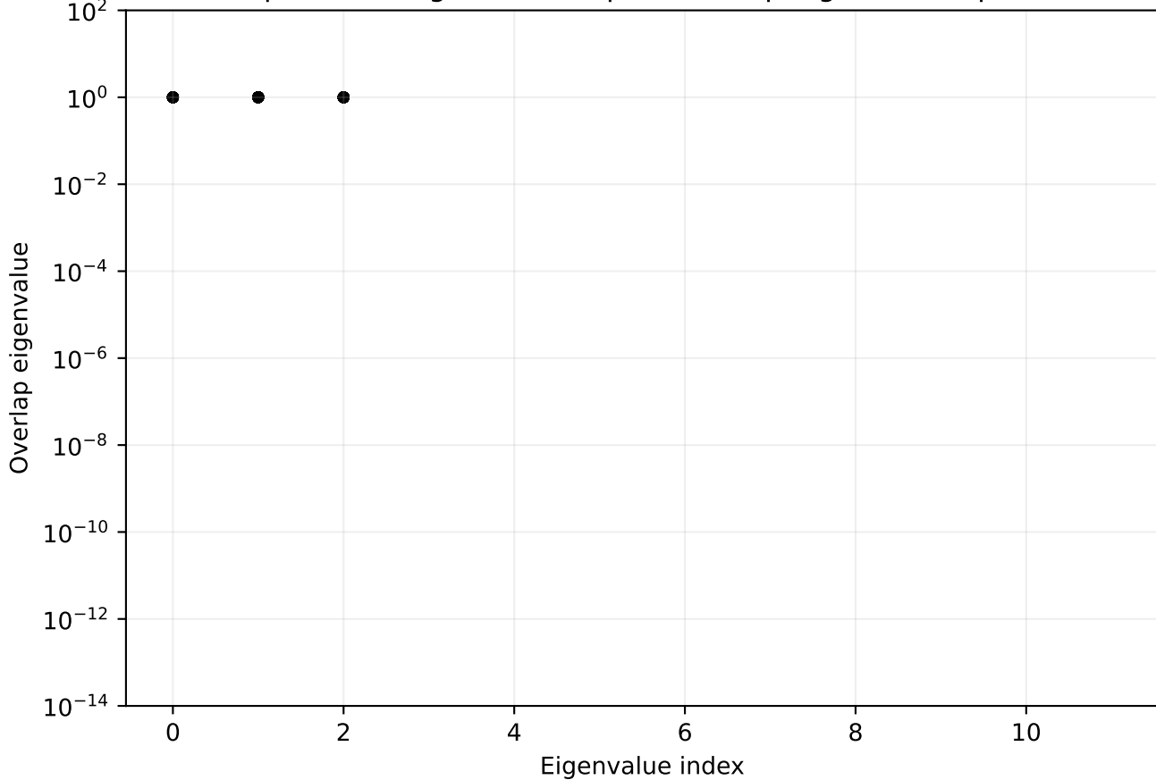
1UpCCGSDSinglet 2e2o Triplet Overlap Eigenvalue Spread
