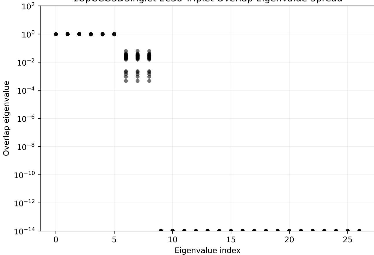
1UpCCGSDSinglet 2e3o Triplet Overlap Eigenvalue Spread
