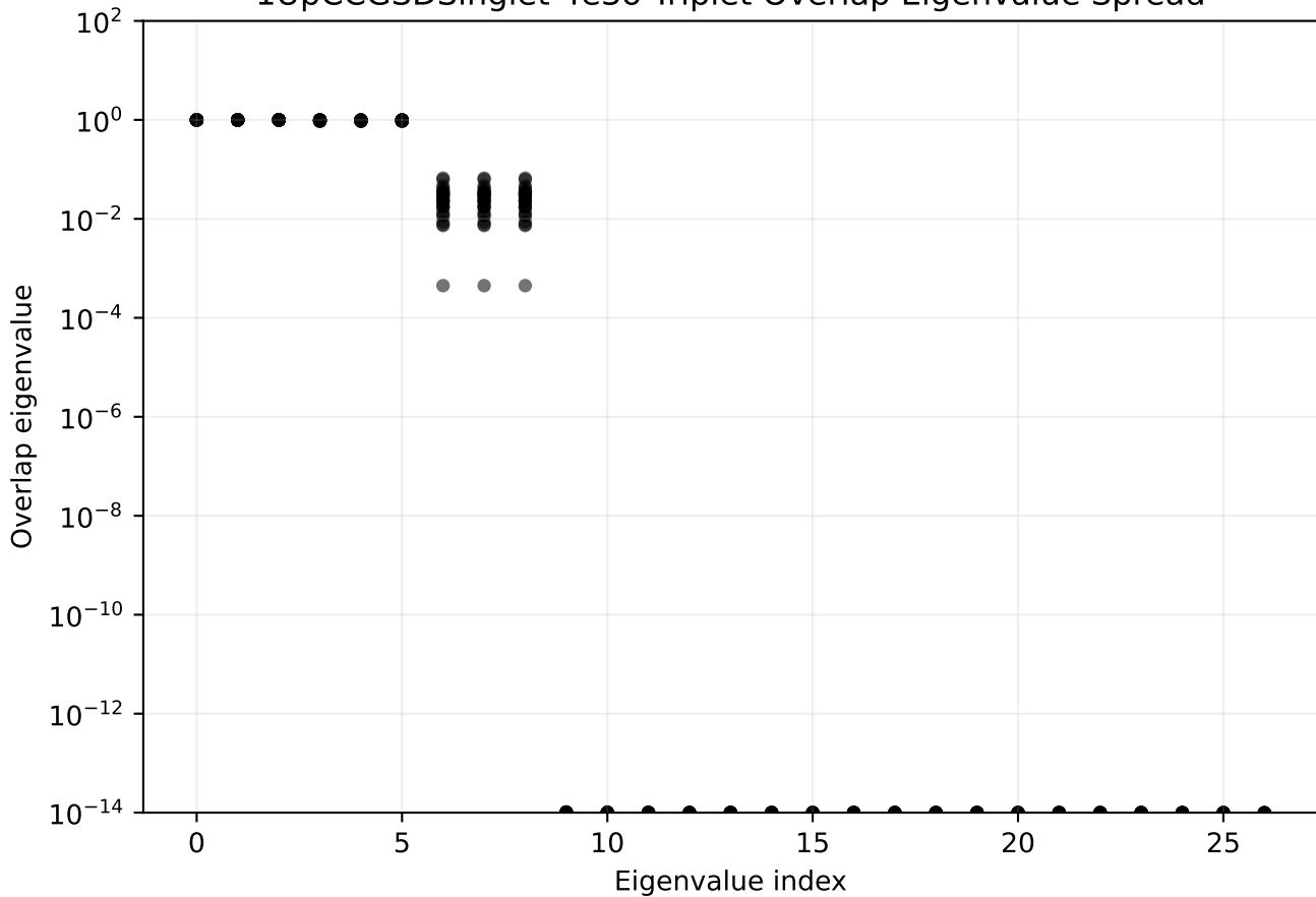
1UpCCGSDSinglet 4e3o Triplet Overlap Eigenvalue Spread
