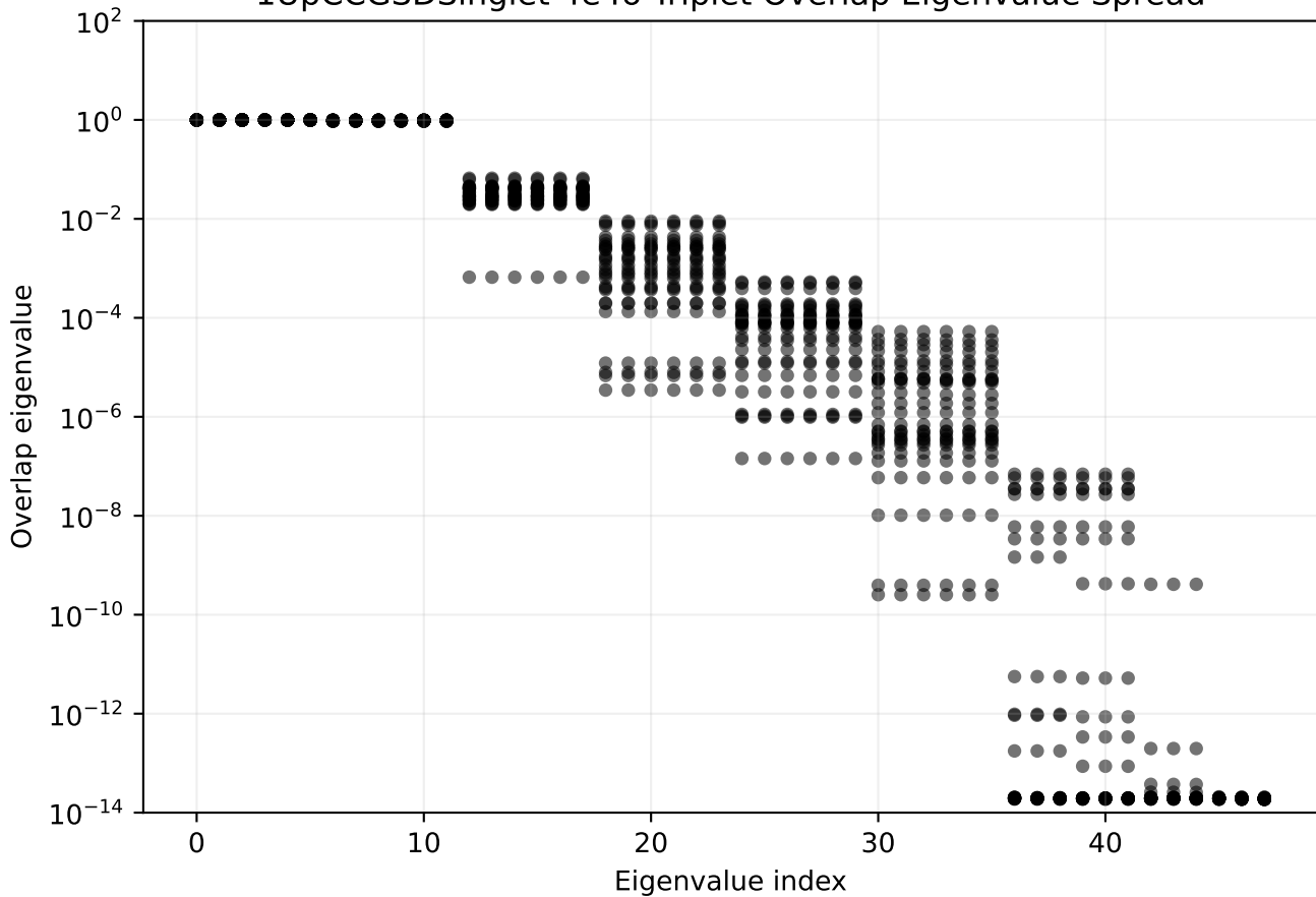
1UpCCGSDSinglet 4e4o Triplet Overlap Eigenvalue Spread
