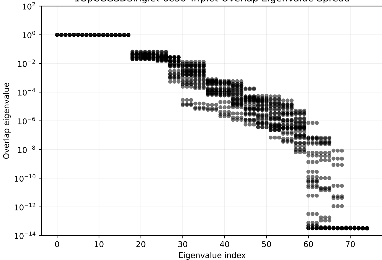
1UpCCGSDSinglet 6e5o Triplet Overlap Eigenvalue Spread
