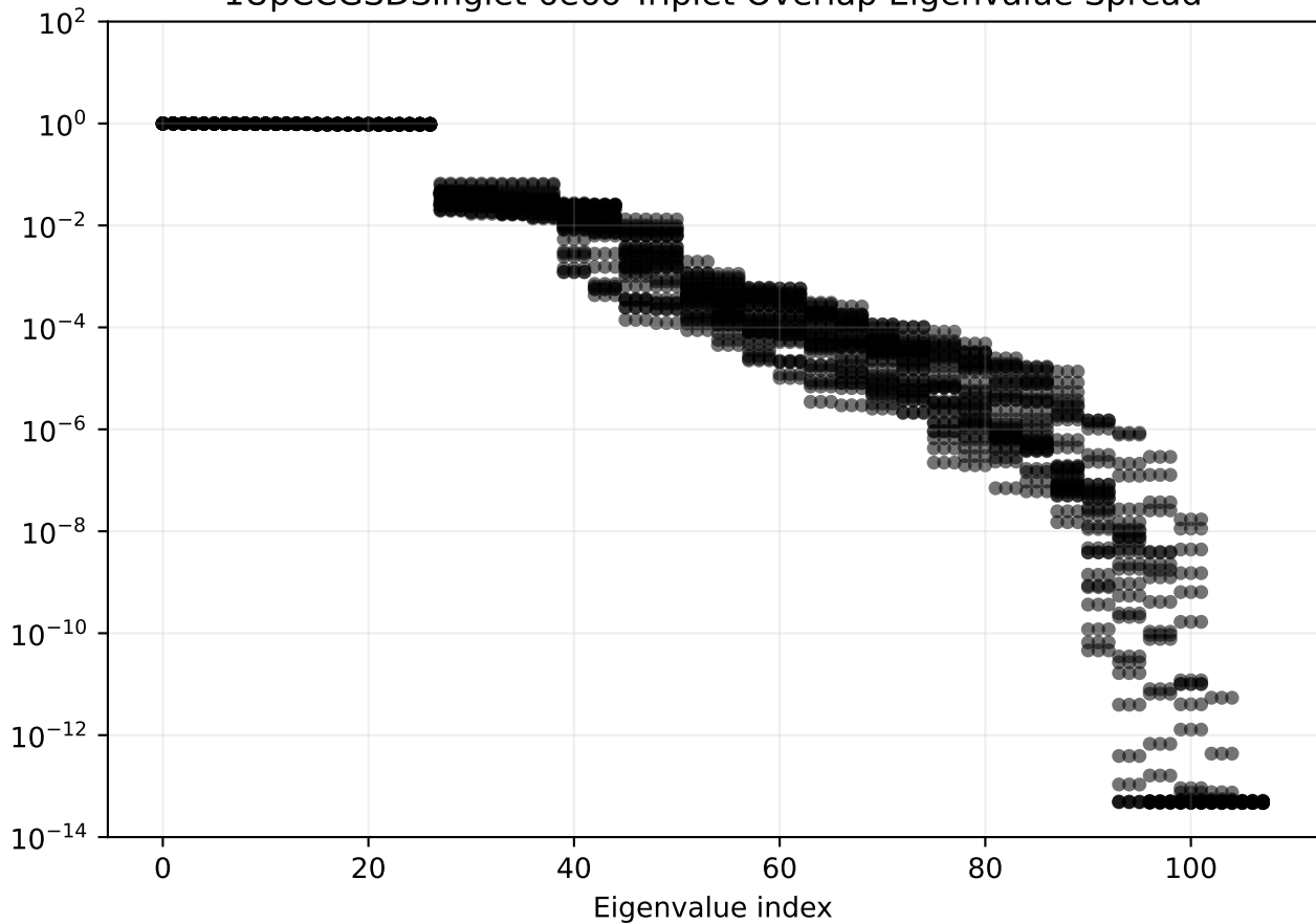
1UpCCGSDSinglet 6e6o Triplet Overlap Eigenvalue Spread
