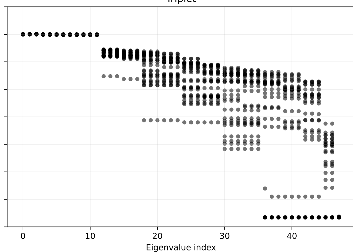
Triplet
