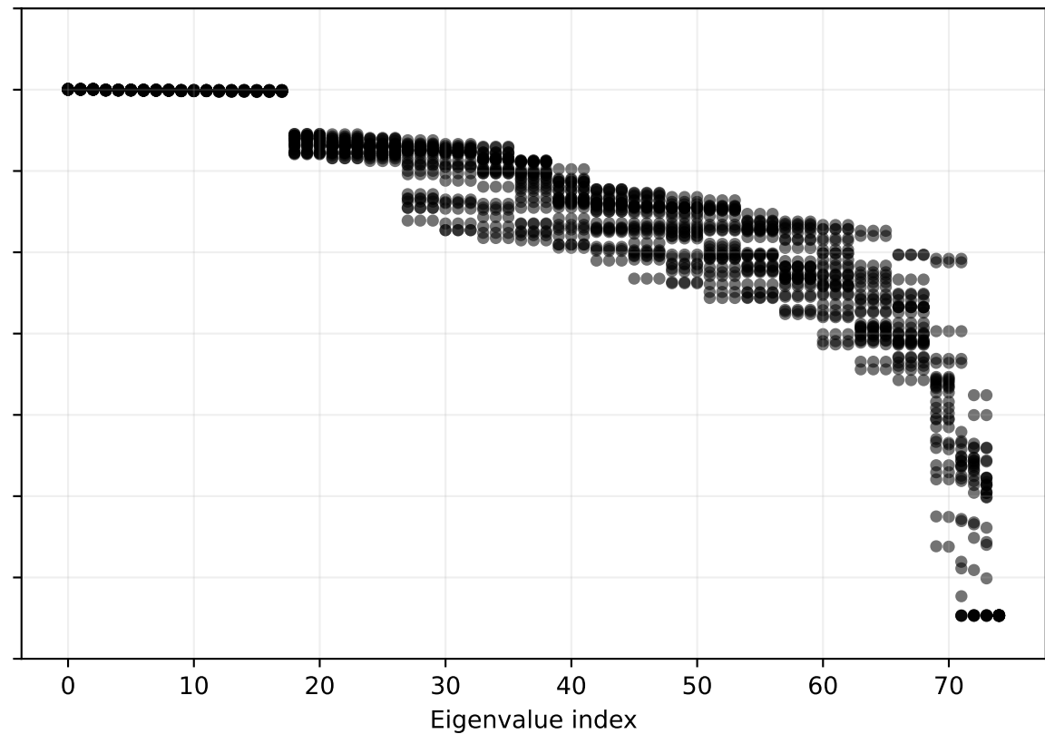
Triplet
