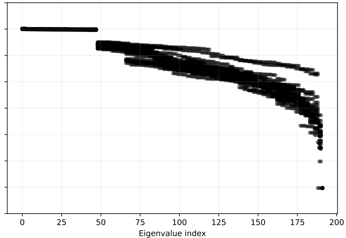
Triplet
