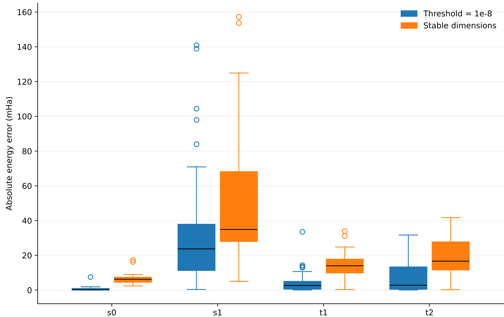
UCCSD 6e6o: Threshold vs Stable QSE Dimensions
