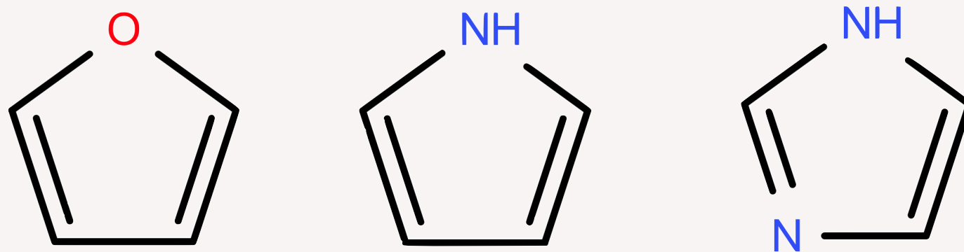
Furan
