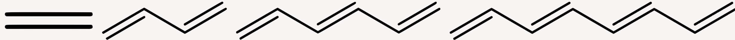
Ethene
