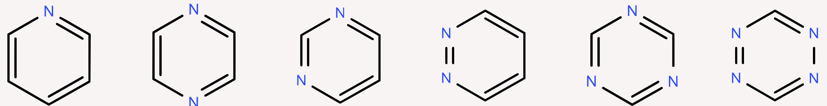
Pyridine
