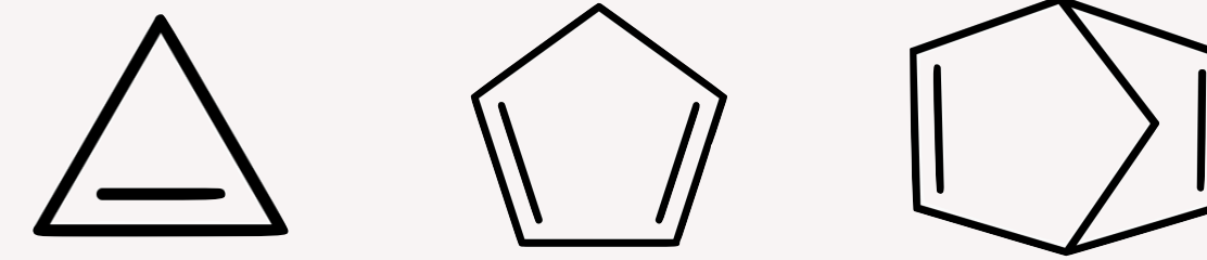
Cyclopropene
