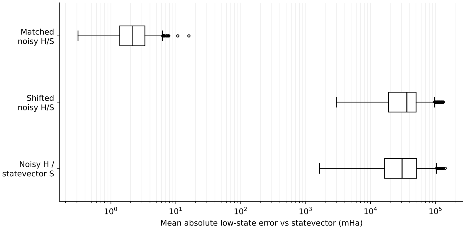
Effect of Breaking H-S Correlated Errors: UCCSD 6e6o, 100k Shots, 1e-2 Threshold
