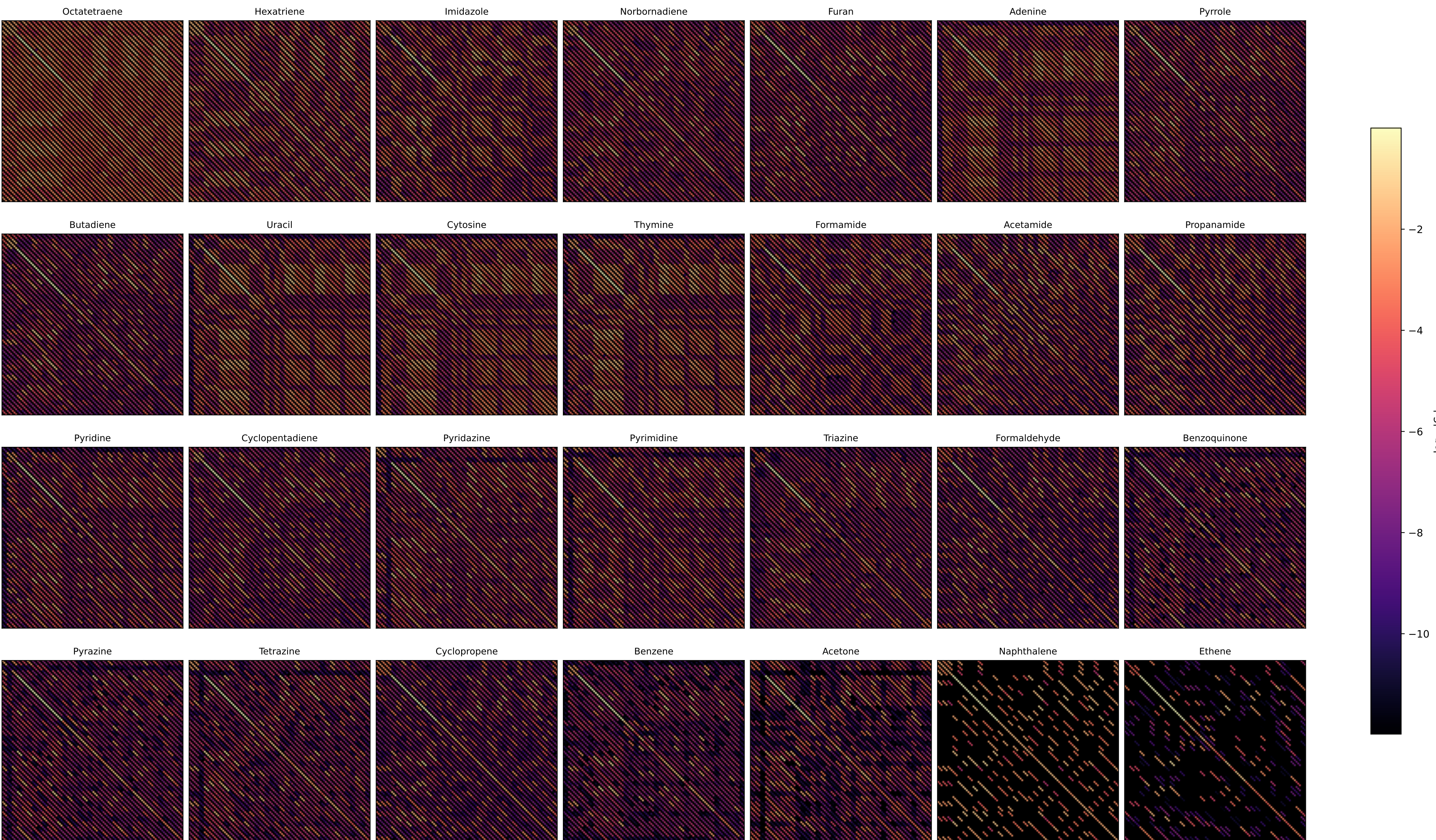
UCCSD 6e6o Triplet Overlap Matrices
