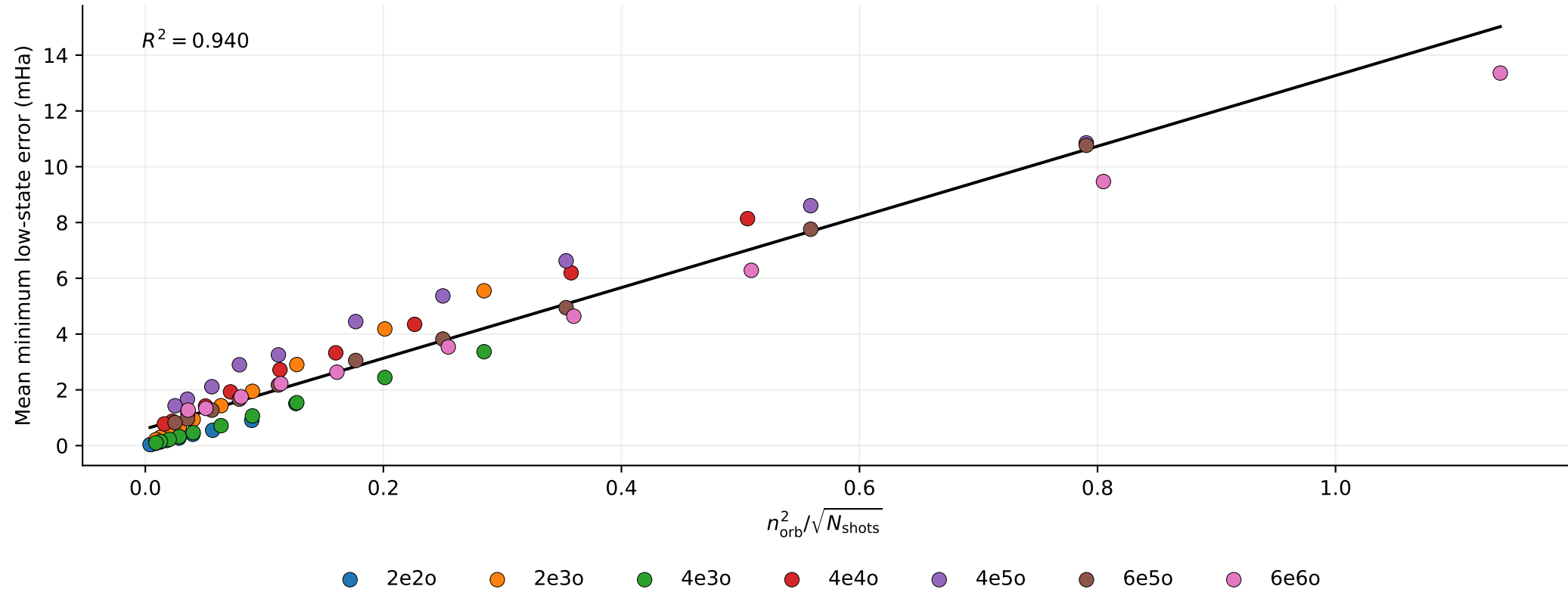
Shot-Noise Scaling of Minimum QSE Error by Active Space
