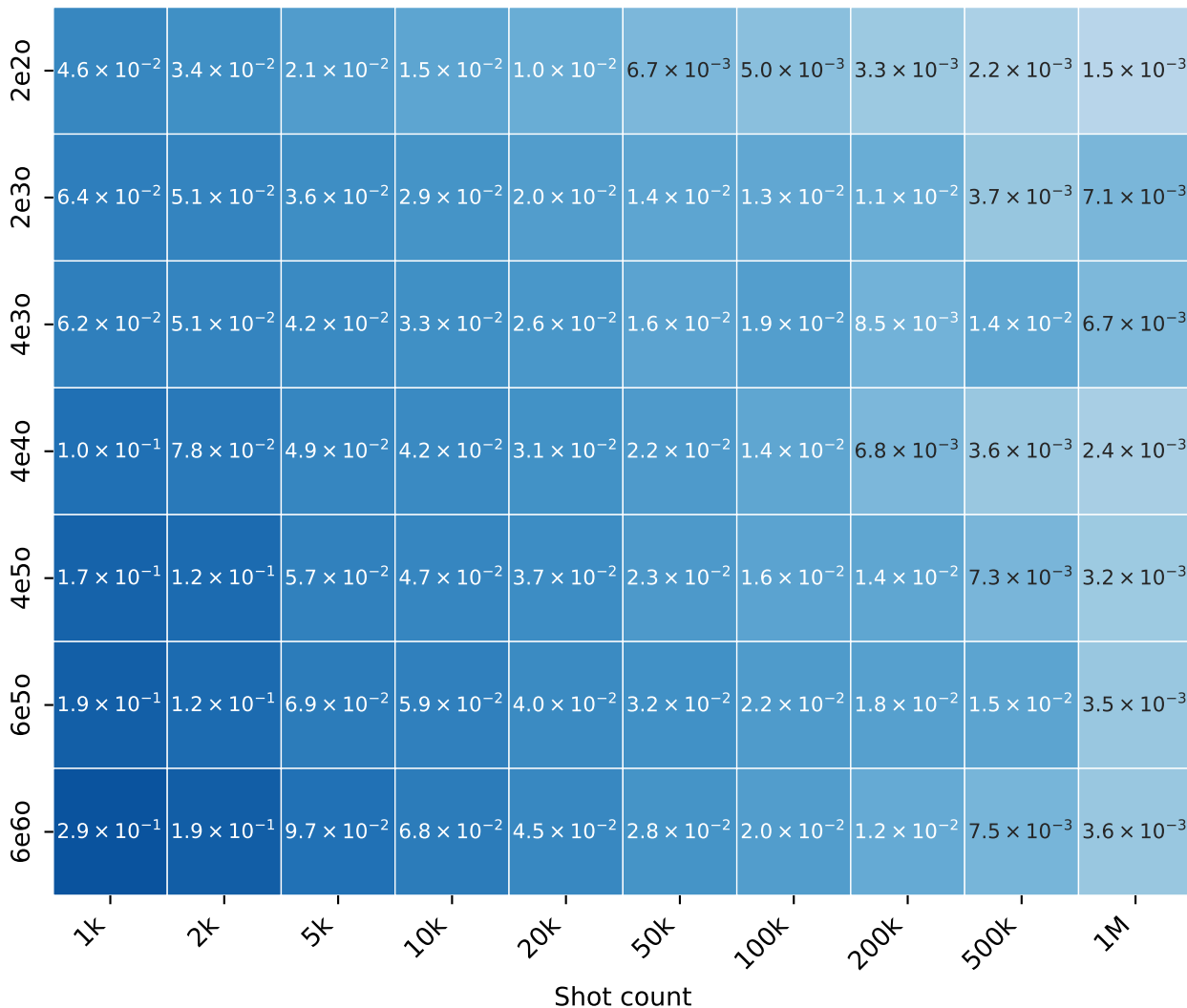
Mean Optimal Threshold by Active Space and Shot Count
