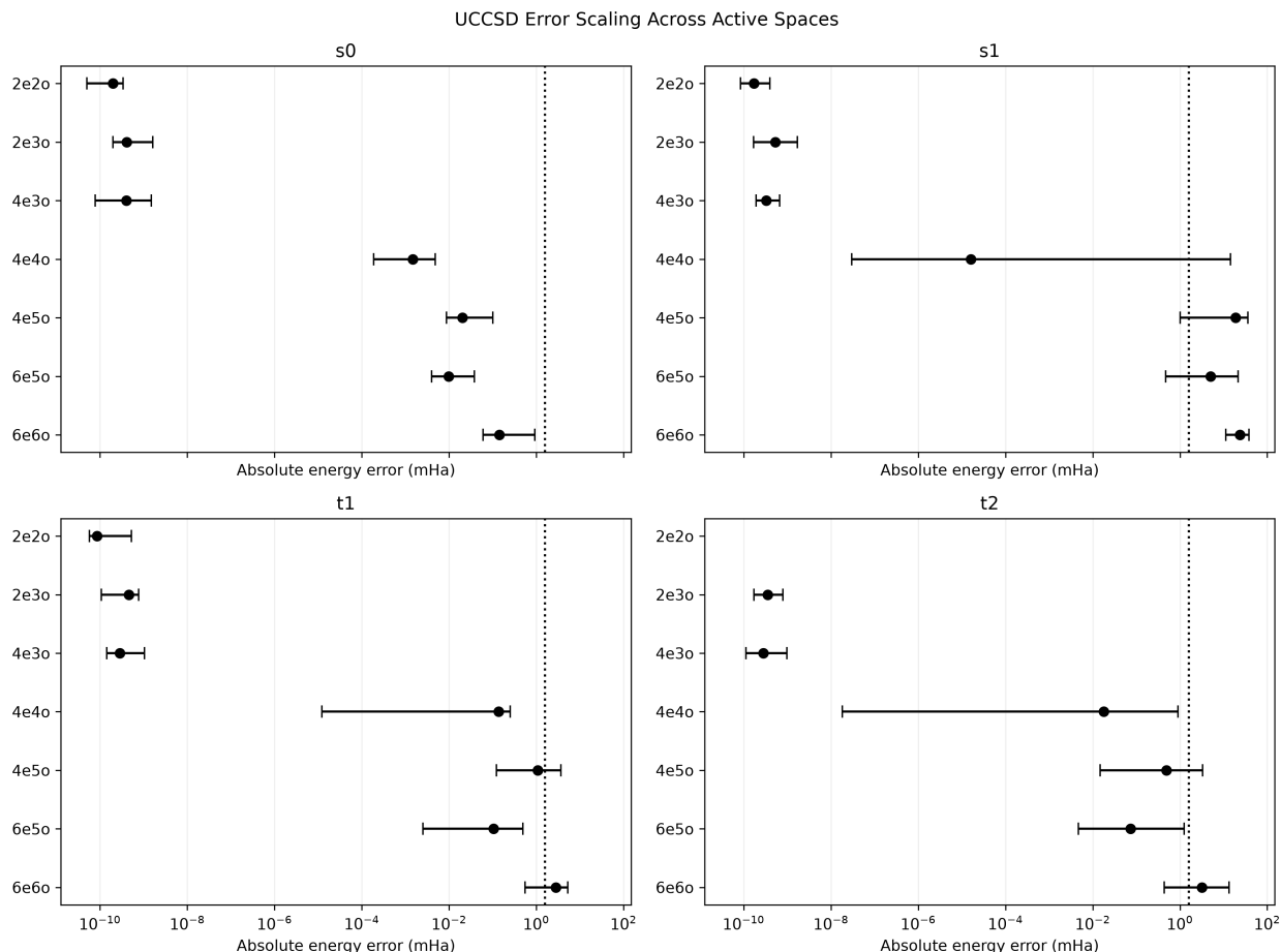
Figure 2: Dependence of UCCSD QSE energy errors on active-space size. Results are shown for the lowest singlet and triplet states across the 2e2o, 2e3o, 4e3o, 4e4o, 4e5o, 6e5o, and 6e6o active spaces. Markers and horizontal error bars summarize the central error and spread across the molecular benchmark, while the dotted line denotes chemical accuracy.
