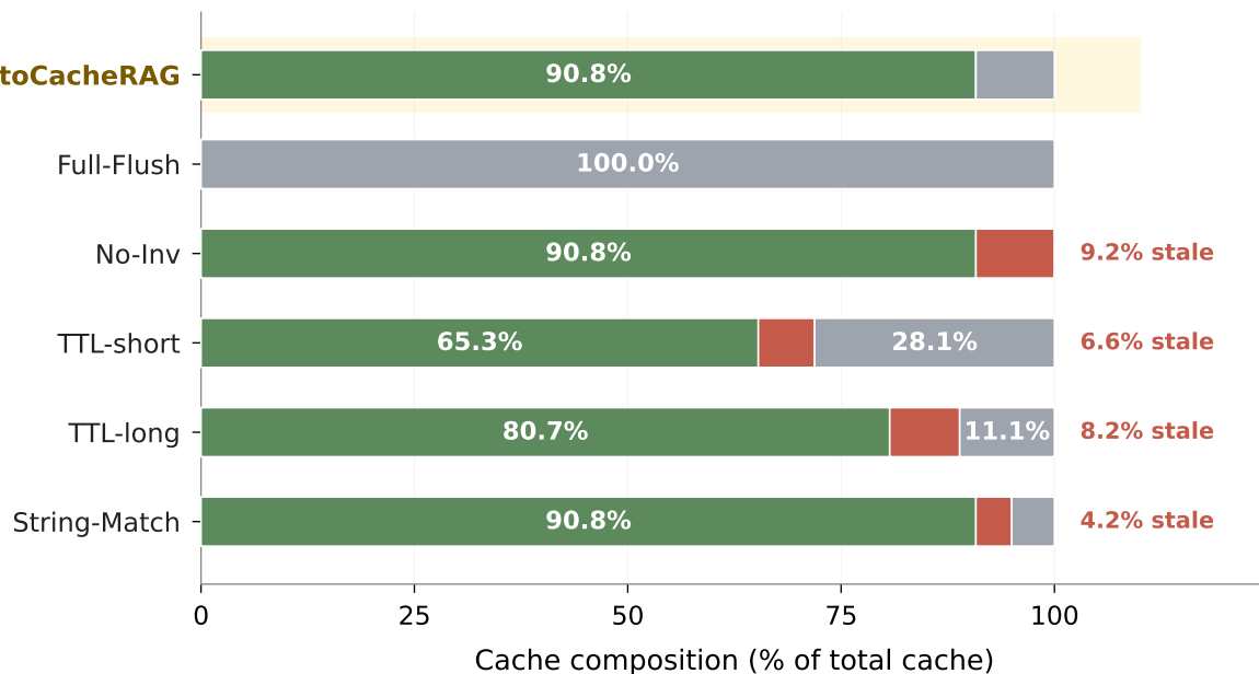
(a) ABox revocation — baseline stale = 9.2%
