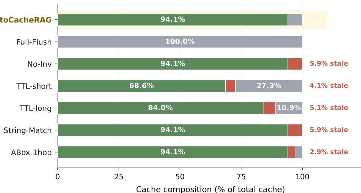
(b) TBox restructuring — baseline stale = 5.9%
