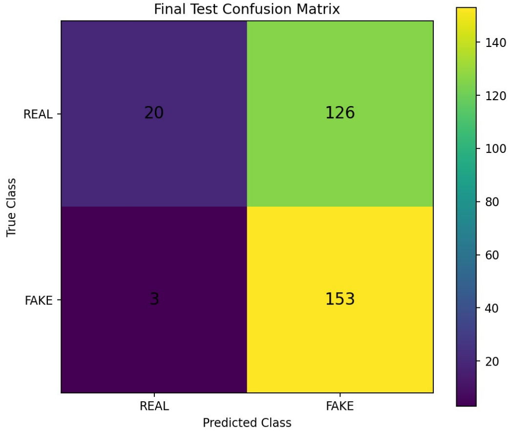
Şekil 3. Nihai test confusion matrix: TN=20 , FP=126 , FN=3 , TP=153 .
