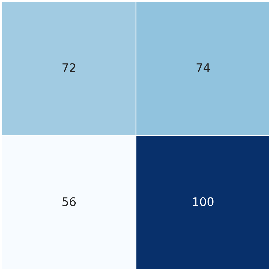
VGG16 + SVM — Test Confusion Matrix
