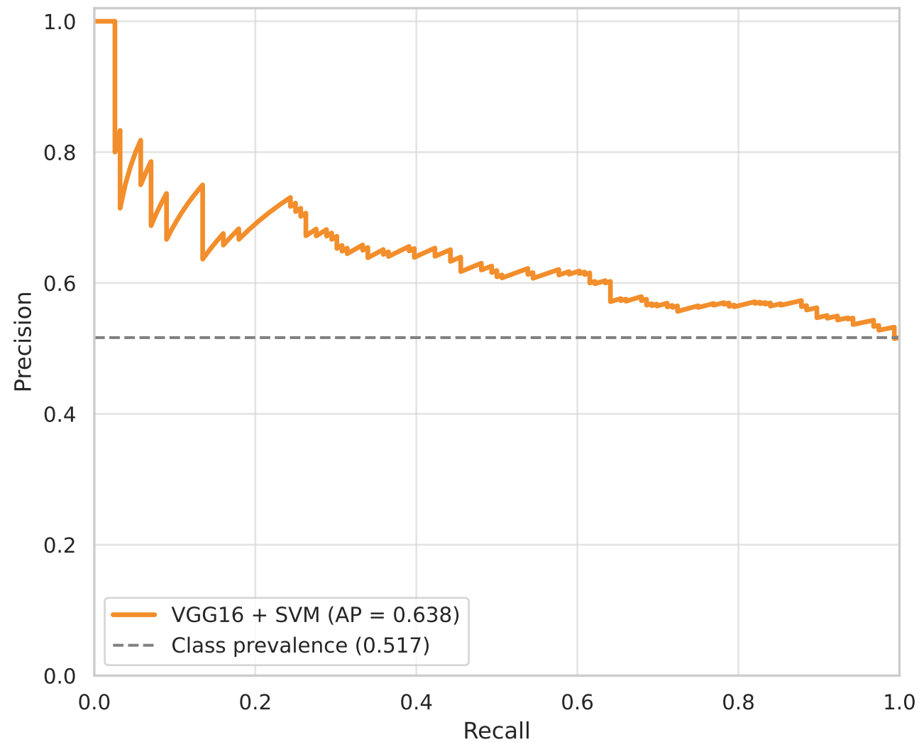
VGG16 + SVM — Test Precision-Recall Curve
