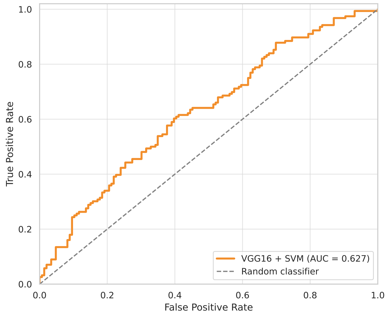
VGG16 + SVM — Test ROC Curve
