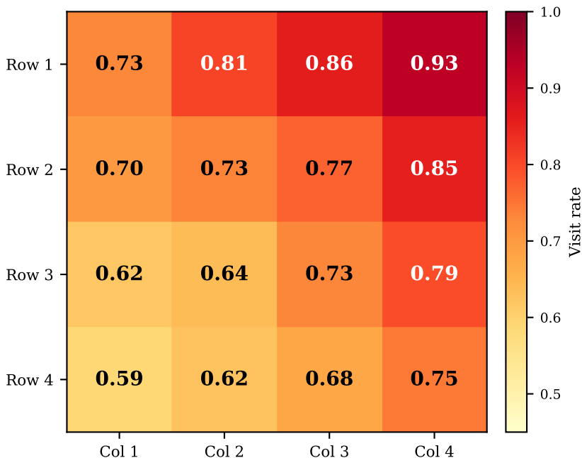
Board Cell Visitation Frequency (fraction of steps with non-empty tile)
