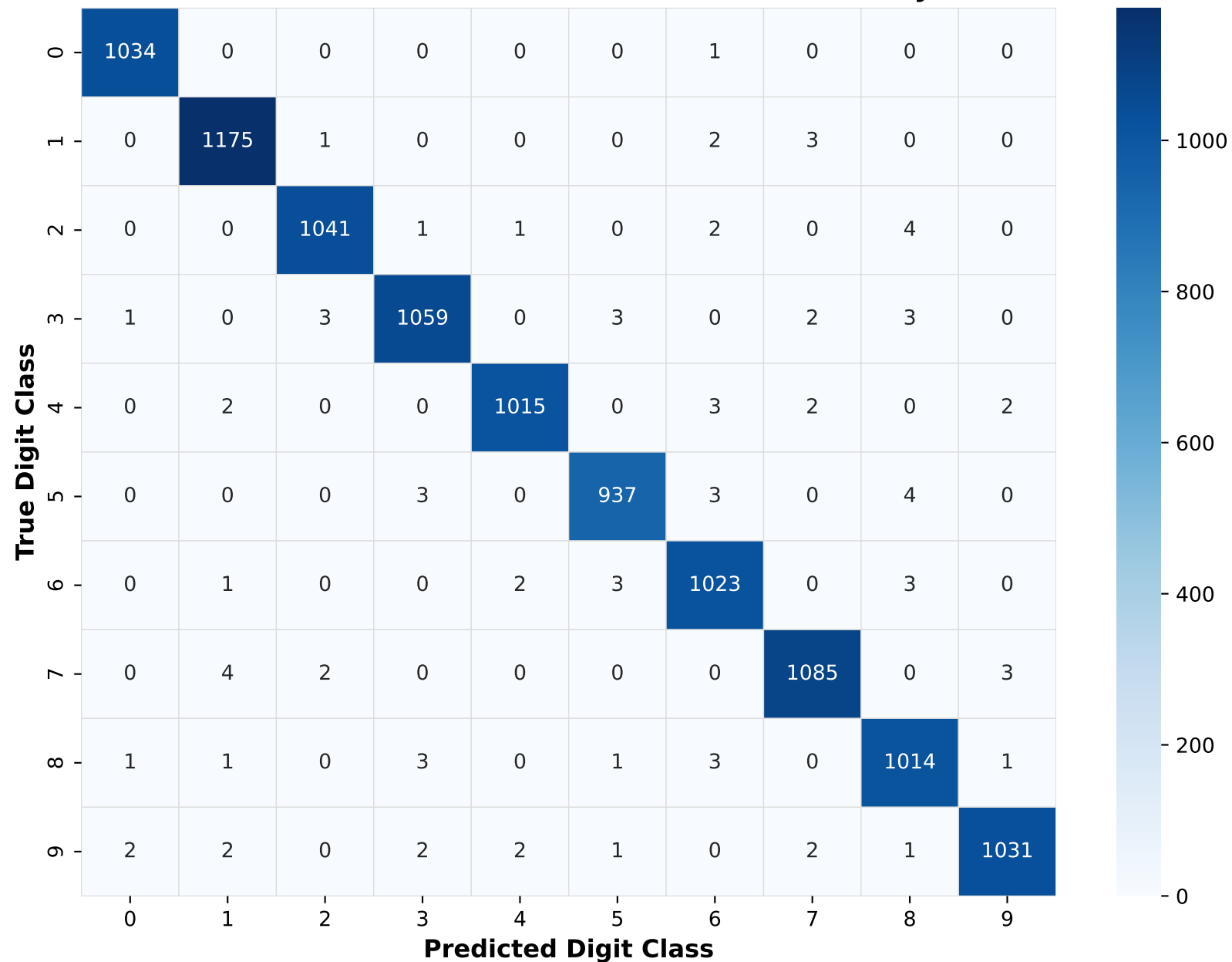
LeNet-5 Baseline: Test Set Confusion Matrix (Accuracy: 99.18%)
