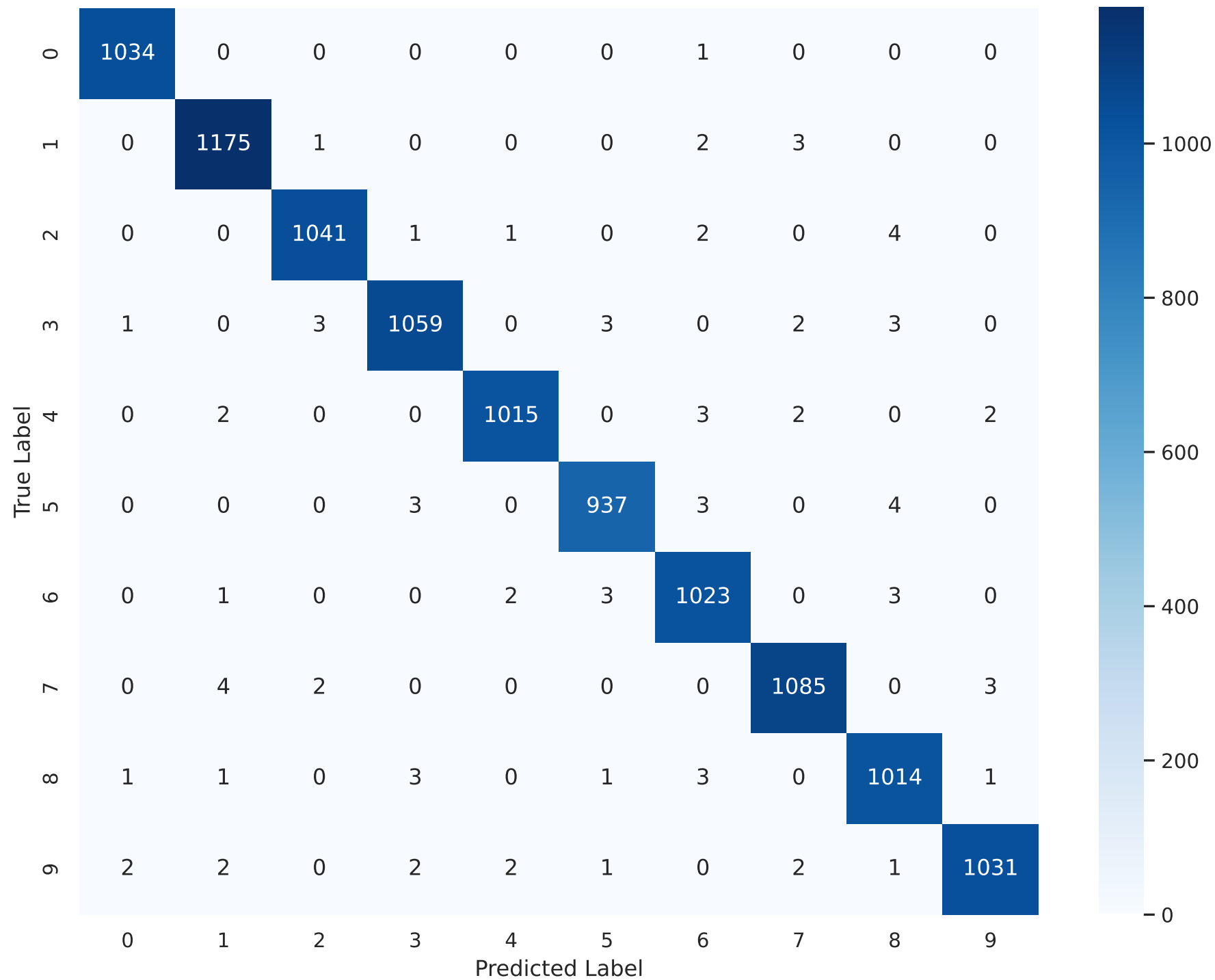
Test Set Confusion Matrix
