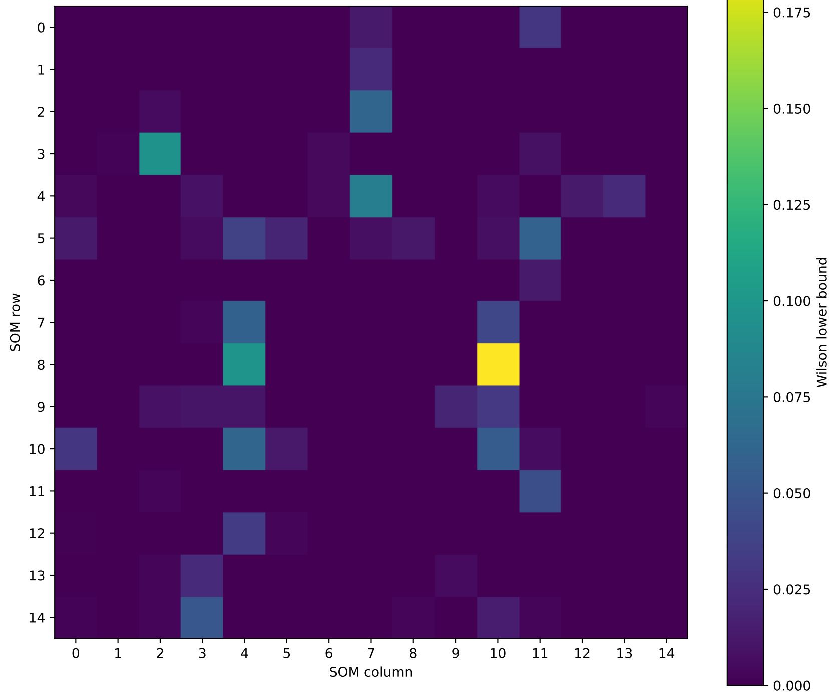
Validation Error Rate: 95% Wilson Lower Bound
