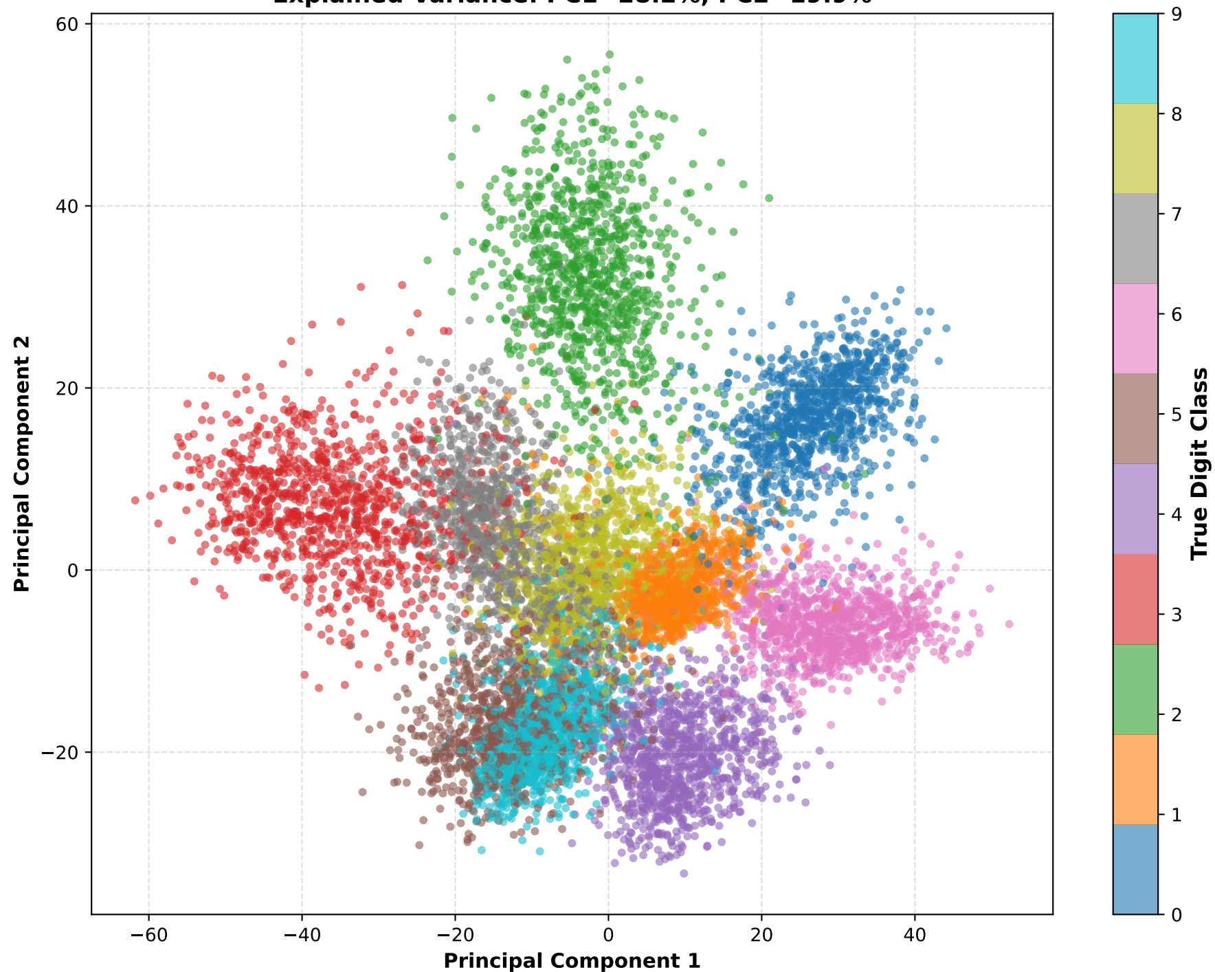
2D PCA Projection of 84-Dimensional fc2 Embeddings (Test Set) Explained Variance: PC1=28.2%, PC2=19.9%
