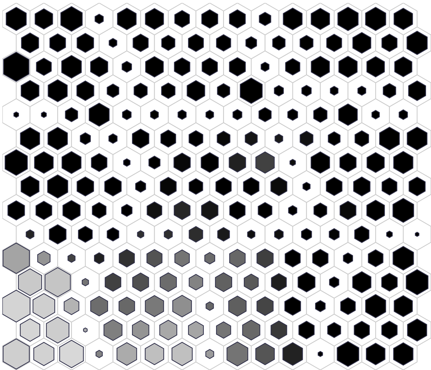
Average LeNet fc2 Feature 79 (Gray Hist)
