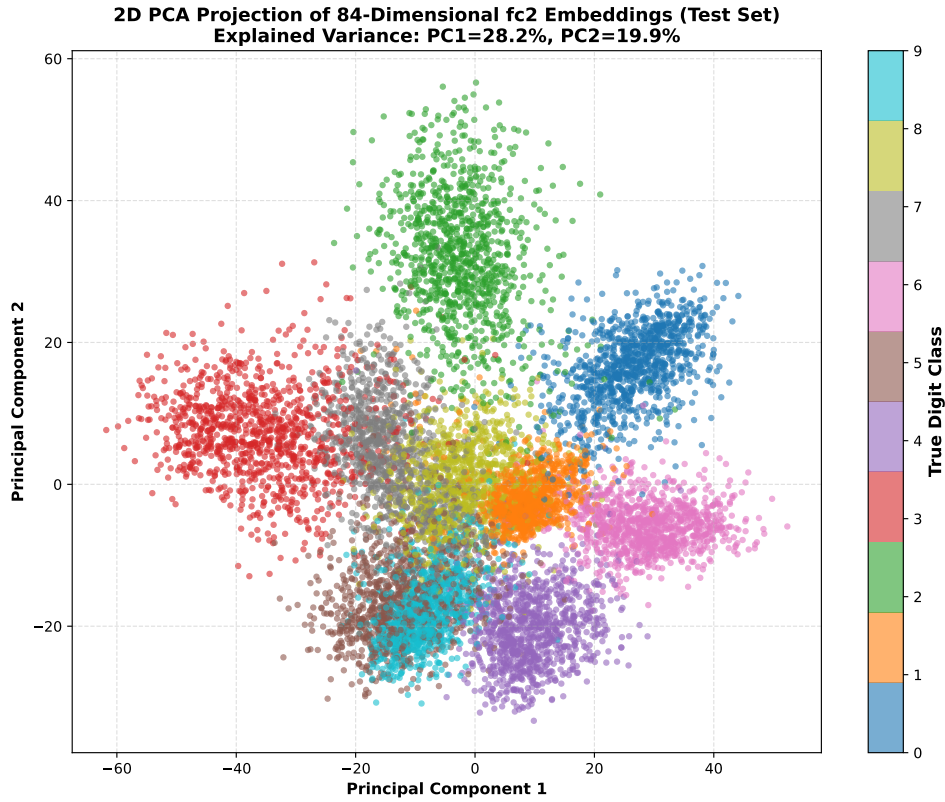
Figure 3. PCA projection of the 84-dimensional fc2 test embeddings for visualization only.
