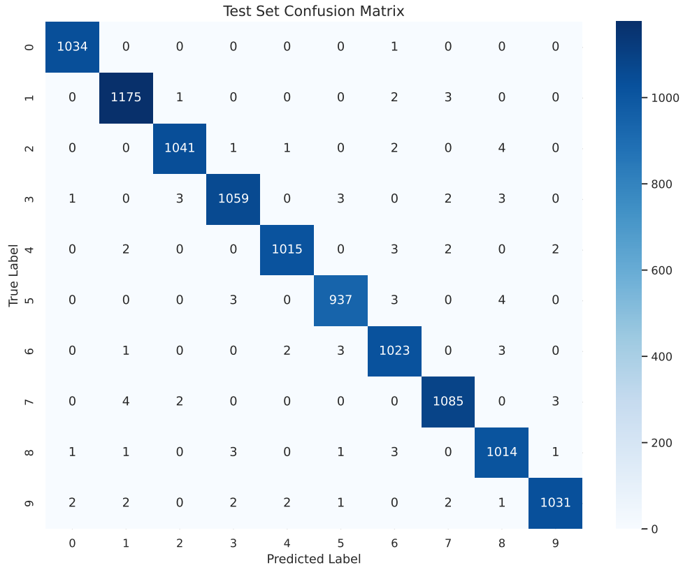
Figure 2. Test-set confusion matrix. The strong diagonal indicates high class-level accuracy.
