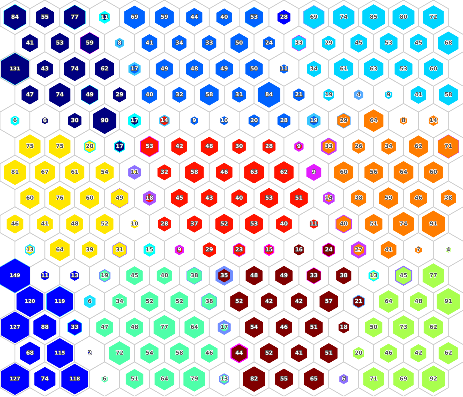
Validation Error Geography — Face: Dominant True Class; Edge: Dominant Wrong Prediction; Width: Error Concentration
