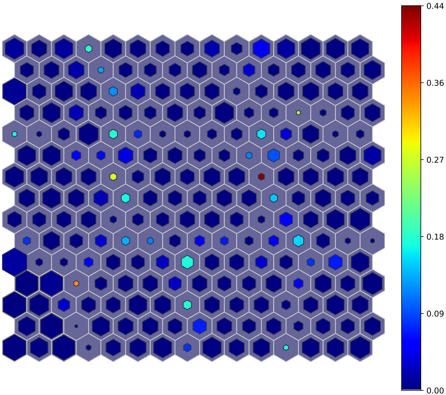
Validation Error Geography — Color: Error Rate; Size: Support
