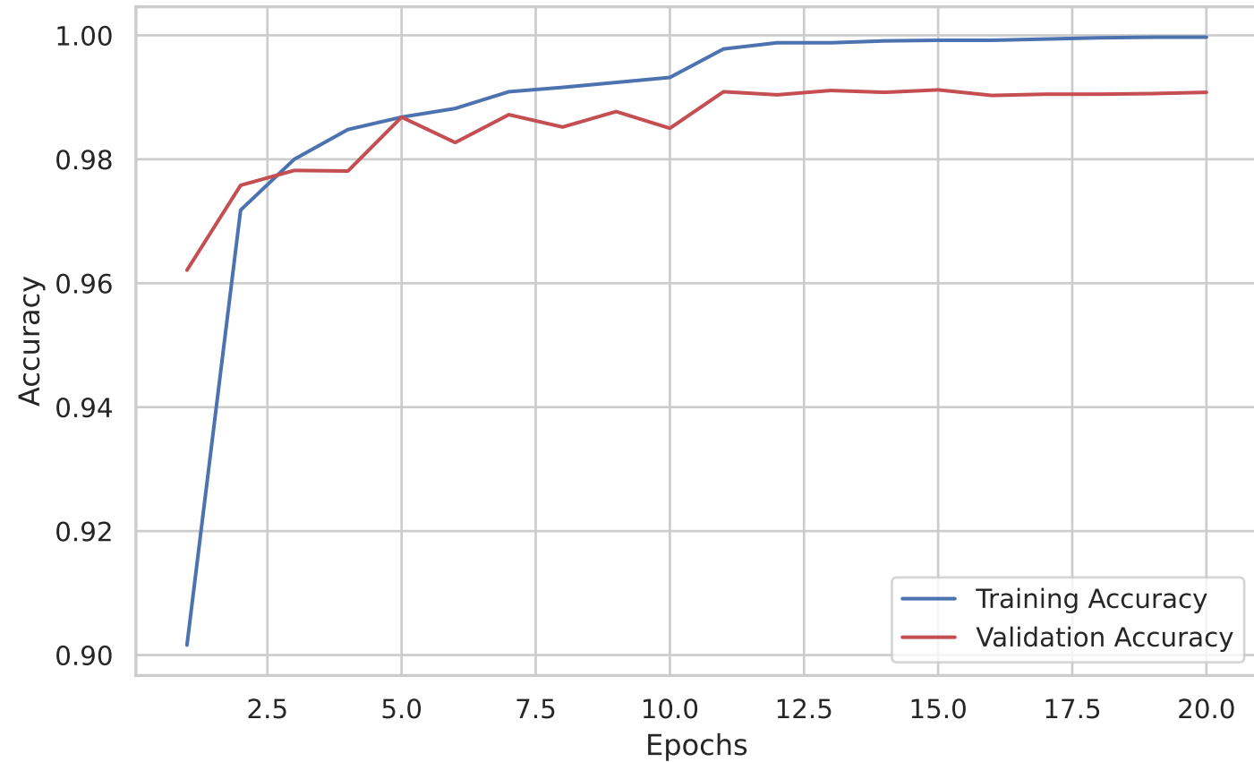
Training and Validation Accuracy
