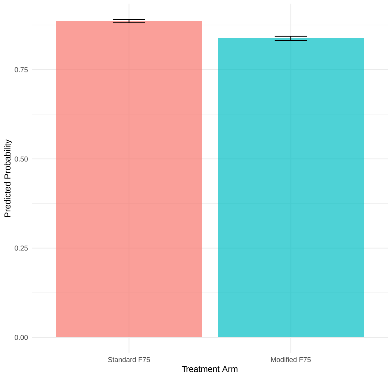
Predicted Probability of Death Before Stabilization
