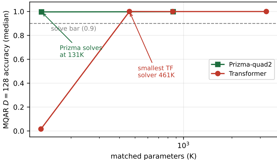
Parameter-efficiency: \geq 3.5\times (131K vs. 461K)
