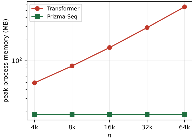
Measured peak (2.8× at 4k → 31× at 64k)
