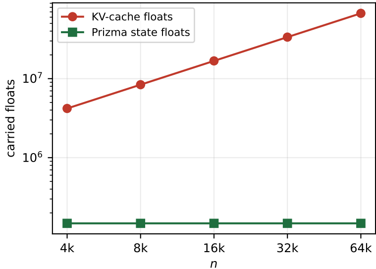
Analytic state vs. KV (28× → 455×)
