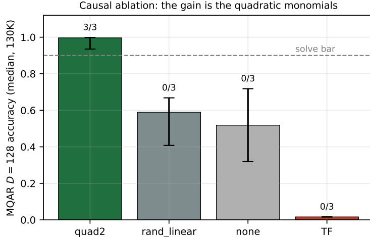
Figure 4: Causal control at 130K (d64L2H2, MQAR D=128 , 3 seeds; error bars span the seed range). Only QUAD2 clears the bar (3/3); rand_linear (a d_\phi=256 random linear lift) behaves like no feature map, and both sit far below QUAD2. The recall gain is the quadratic monomials, not state width. Data: results/gpu_bench.json .
