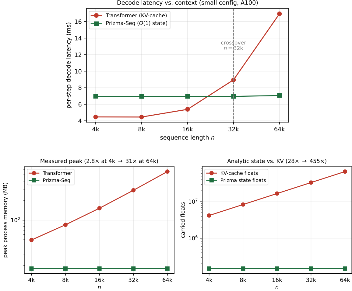
Figure 3: Inference profile (A100, small config). Top: per-step decode latency is flat for Prizma-Seq and crosses the Transformer at n=32k . Bottom: the carried state is constant in n — 28–455× fewer floats than the KV-cache (right, analytic) and 2.8–31× less measured peak memory (left). Data: results/gpu_latency.json .
