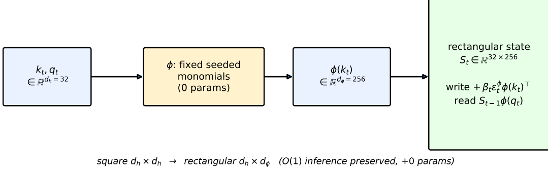
Figure 1: The QUAD2 lift makes the per-head delta-state rectangular ( d_h \times d_\phi ) at zero added parameters; the per-token write and read stay matrix–vector products over a state whose size d_h d_\phi is independent of the sequence length n , so O(1) inference is preserved.
