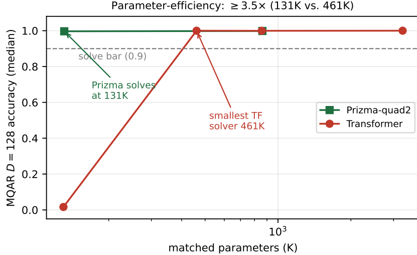
Figure 2: MQAR ( D=128 ) median accuracy vs. matched parameters (3 seeds; 5 for the 857K TF). Prizma-quad2 solves at 131K where the param-matched Transformer fails (0.016); the smallest Transformer solver on the coarse grid \{130, 461, 857, 3300\} K is d128L2H4 at 461K, giving a \geq 3.5\times parameter-efficiency gap. All points trace to results/gpu_bench.json .
