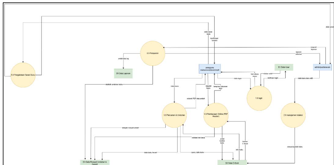
Gambar 5. 2 Dfd Level 1
