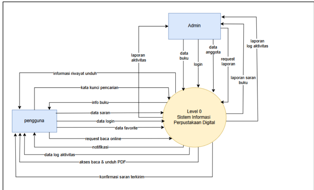
Gambar 5. 1 Dfd Level 0
