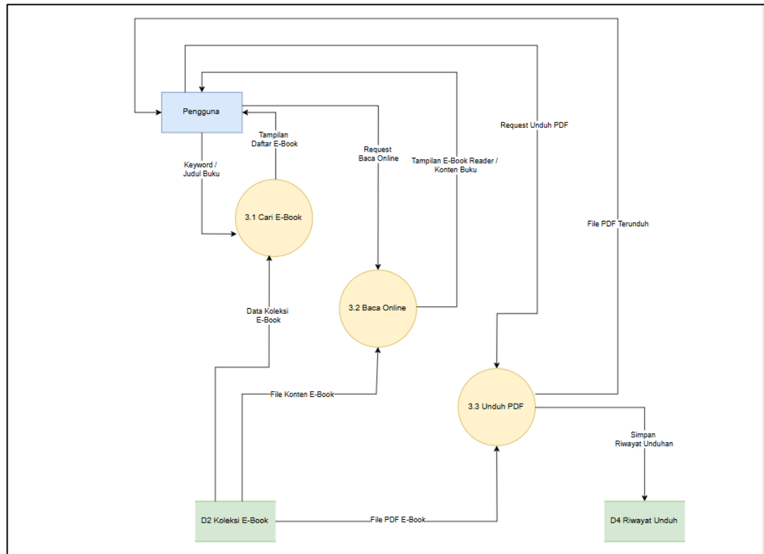
Gambar 5. 5 Dfd Level 2 Proses 3
