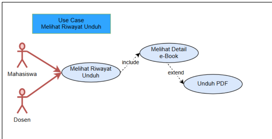
Gambar 4. 6 Use Case Riwayat Unduh
