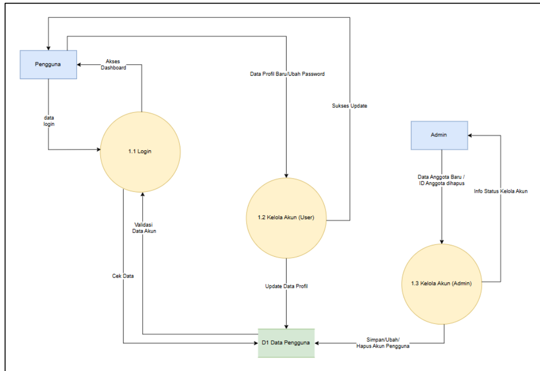
Gambar 5. 3 Dfd Level 2 Proses 1
