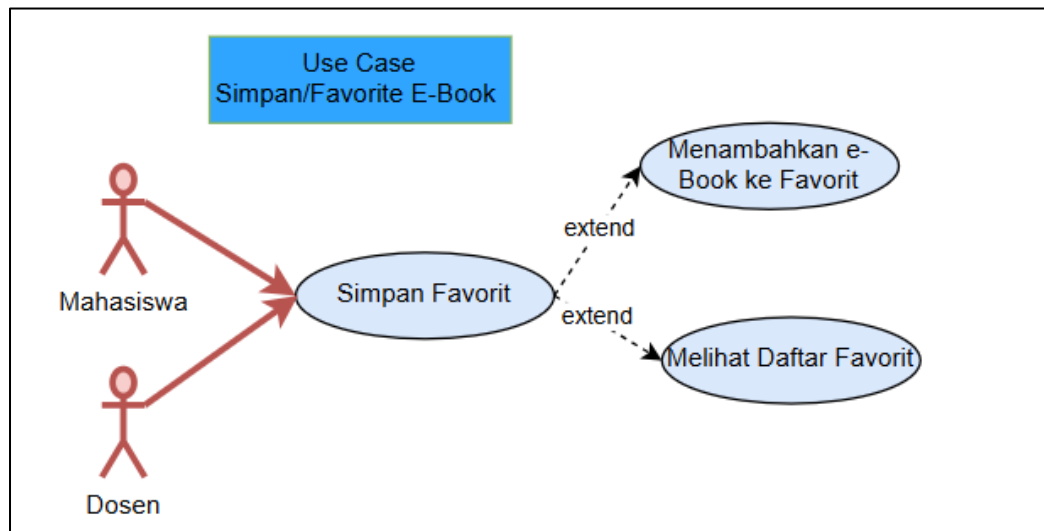
Gambar 4. 5 Use Case Simpan E-Book
