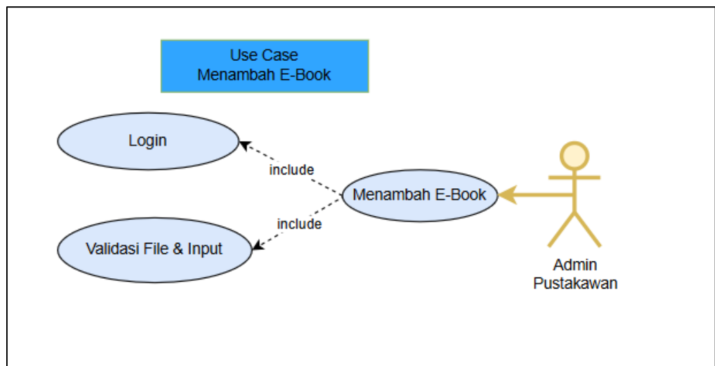
Gambar 4.15 Use Case Menambah E-Book
