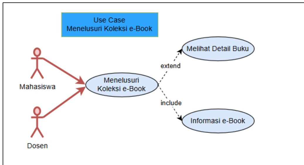
Gambar 4. 2 Use Case Menelusuri Koleksi E-Book
