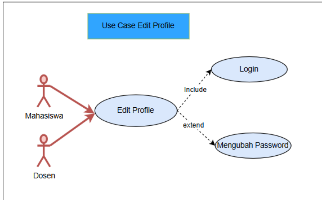
Gambar 4.11 Use Case Edit Profile
