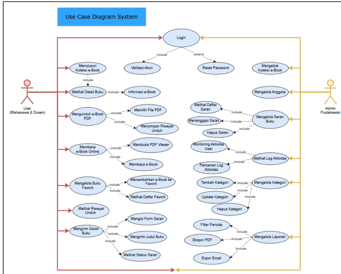
Gambar 3. 1 Use Case
