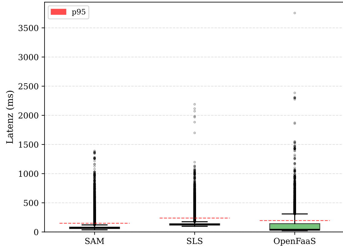
T2 - GET /vehicles Latenz
