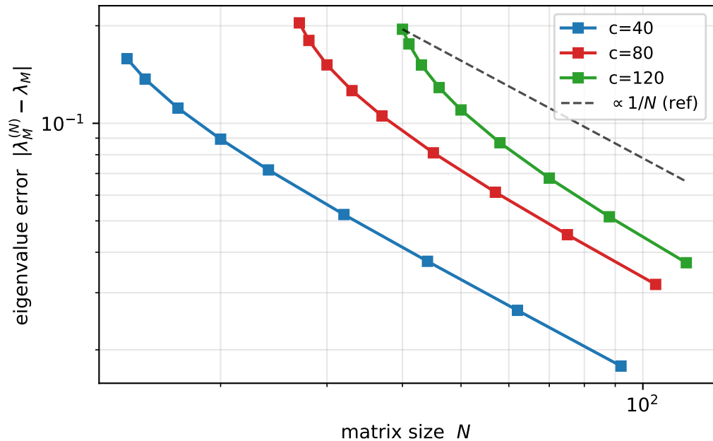
Plunge knee ( m = M ): algebraic \sim 1/N ( n=0 )
