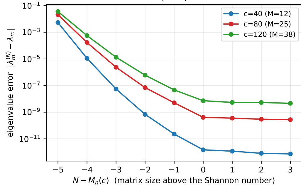
Plateau mode ( m = M-6 ): super-exponential ( n=0 )
