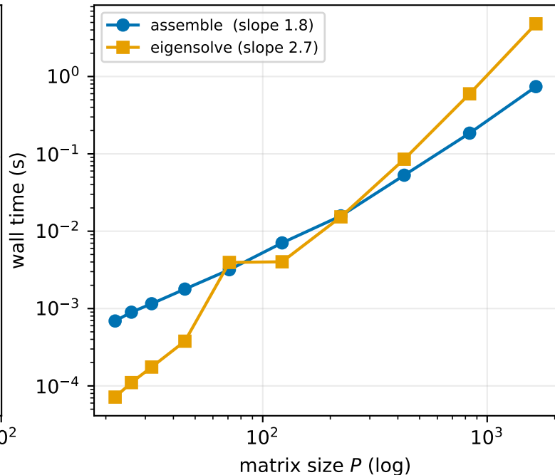
(b) Cost profile vs. matrix size
