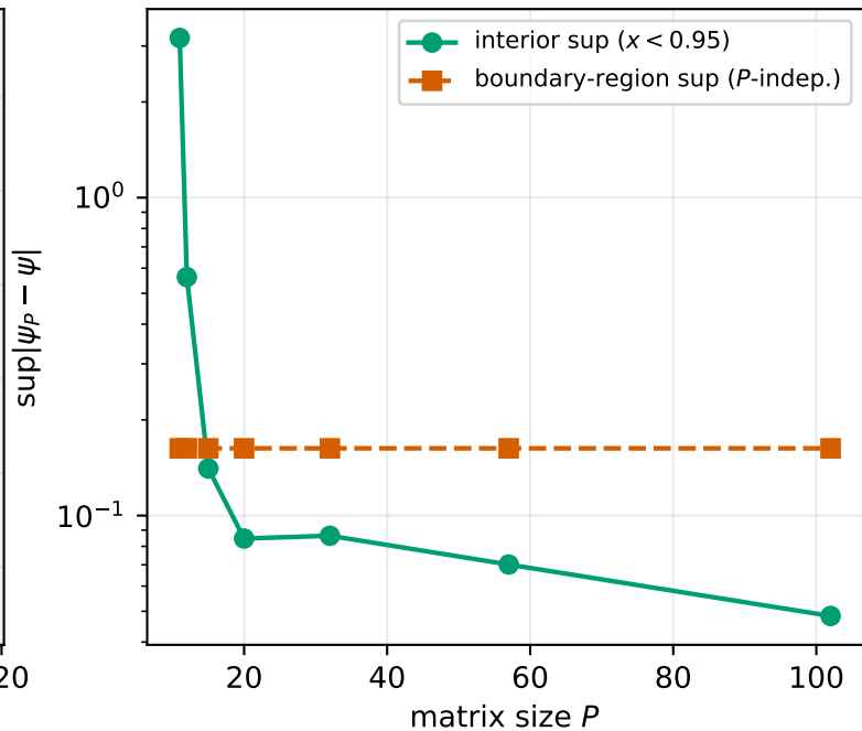
(b) Reconstruction sup-norm: interior vs. FB edge ( n = 0, c = 40 )
