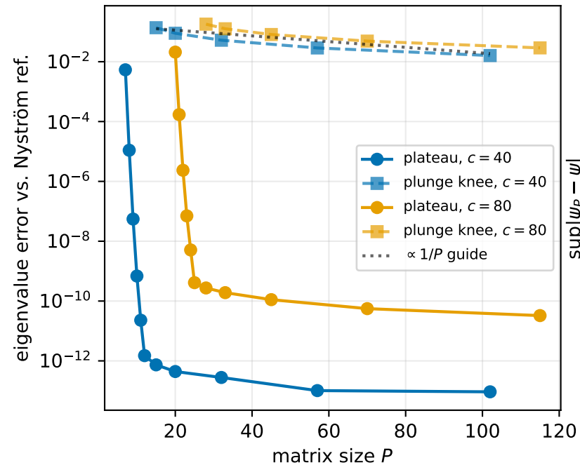
(a) Two-rate eigenvalue convergence
