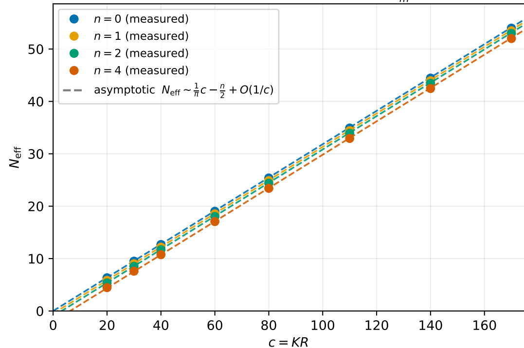
(a) Effective dimension N_{\text{eff}}(n, c) = \sum_m \lambda_m
