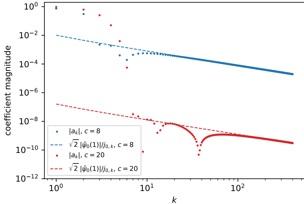
(a) two-regime coefficient decay, m = 0
