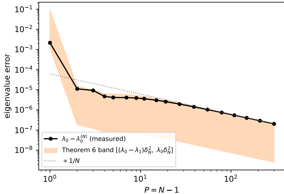
(b) eigenvalue-error crossover, n = 0, c = 8
