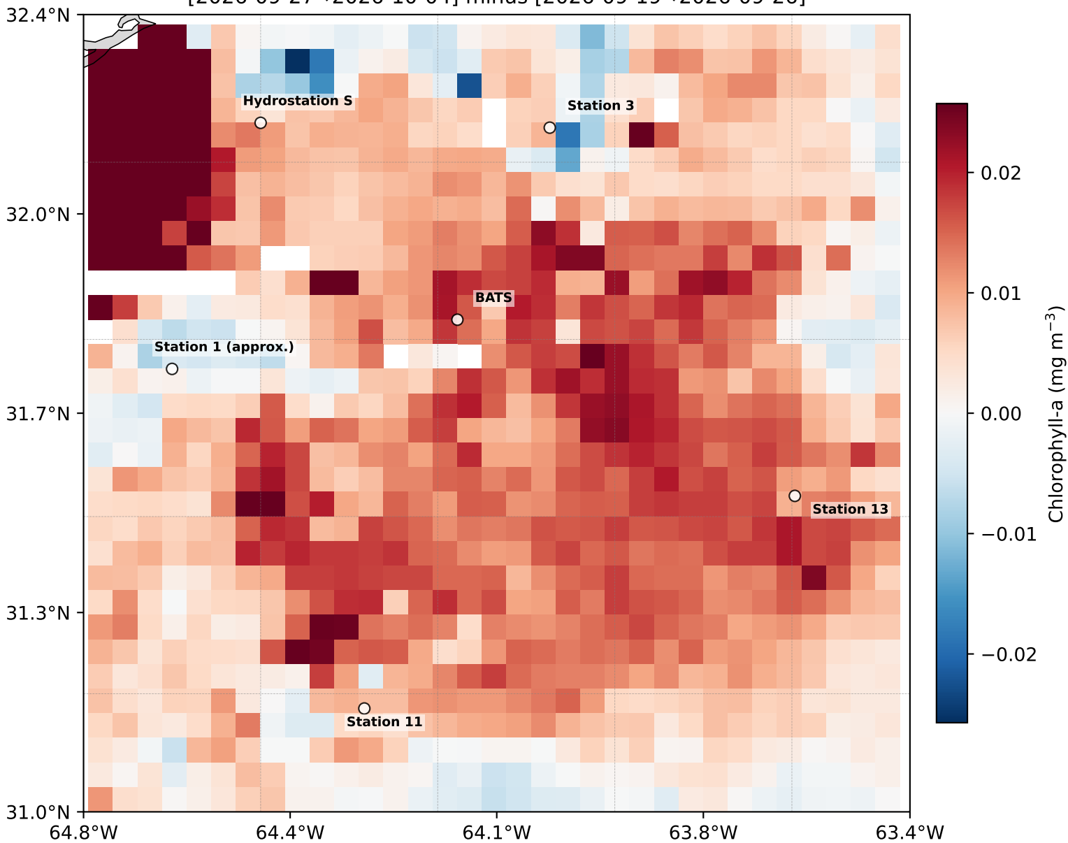
BIOS-SCOPE AE2624 | \Delta CHL (current 8d – previous 8d) [2026-09-27→2026-10-04] minus [2026-09-19→2026-09-26]
