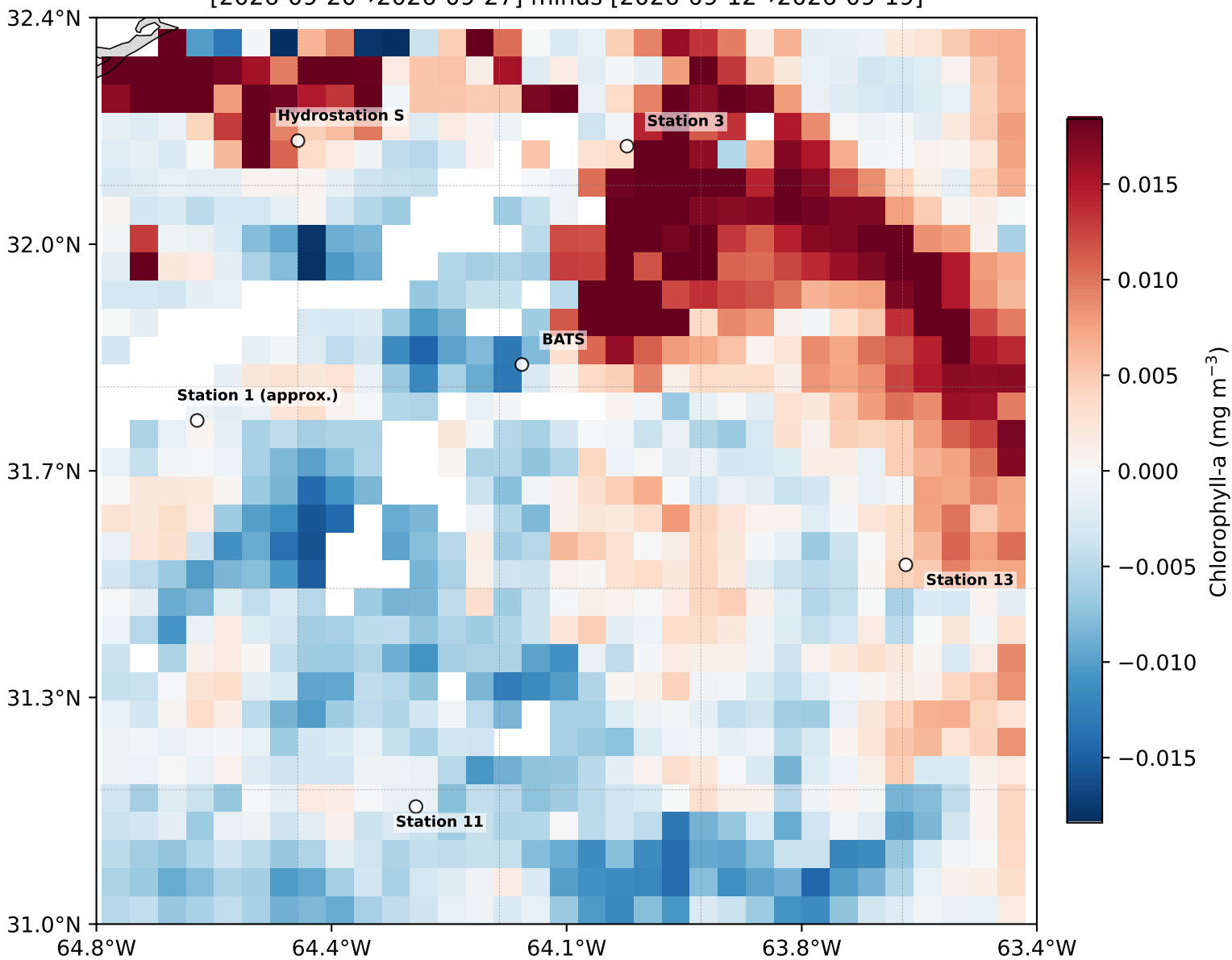
BIOS-SCOPE AE2624 | \Delta CHL (current 8d – previous 8d) [2026-09-20→2026-09-27] minus [2026-09-12→2026-09-19]
