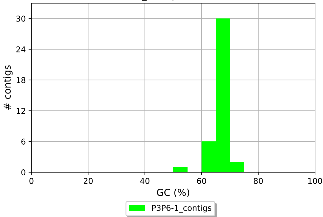
P3P6-1_contigs GC content
