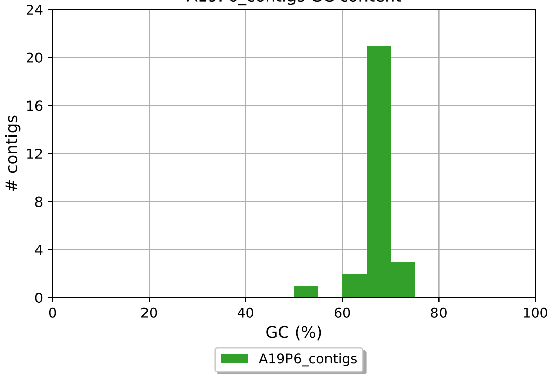
A19P6_contigs GC content
