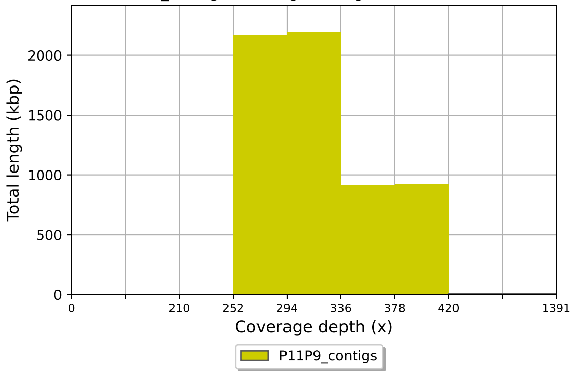
P11P9_contigs coverage histogram (bin size: 42x)
