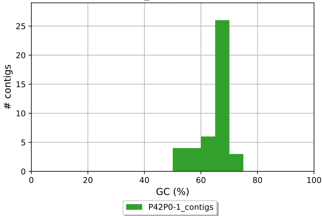
P42P0-1_contigs GC content
