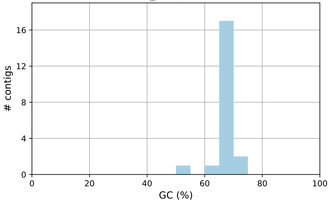
P11P12-1_contigs GC content
