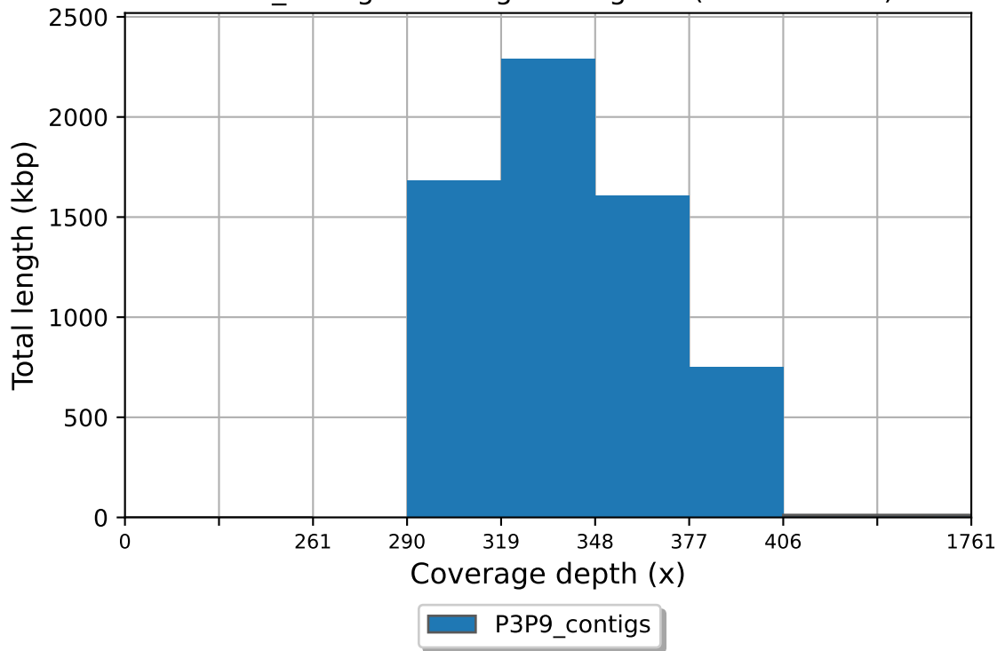
P3P9_contigs coverage histogram (bin size: 29x)
