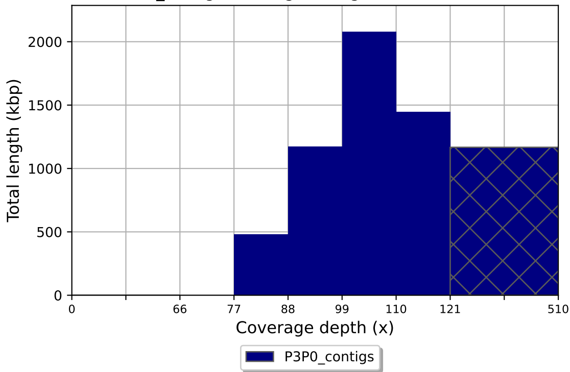
P3P0_contigs coverage histogram (bin size: 11x)
