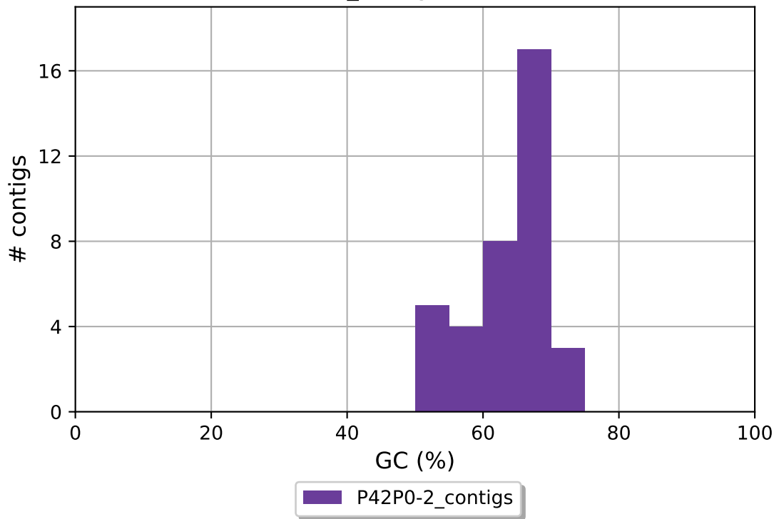
P42P0-2_contigs GC content
