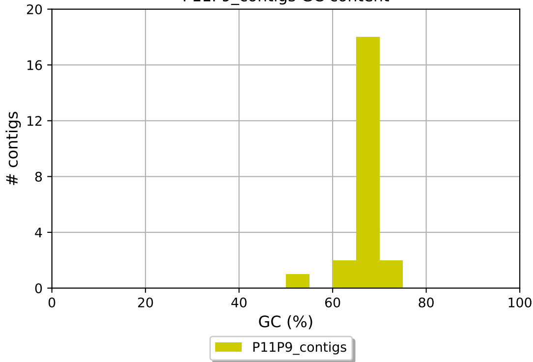
P11P9_contigs GC content
