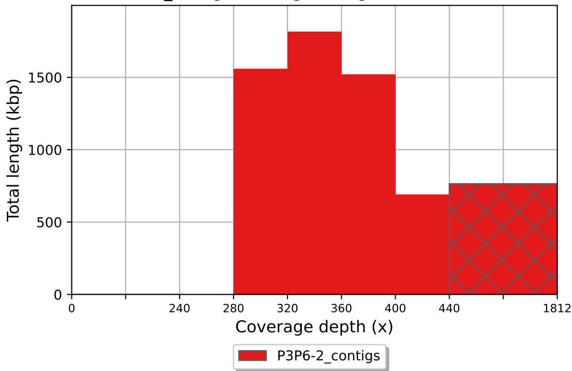
P3P6-2_contigs coverage histogram (bin size: 40x)
