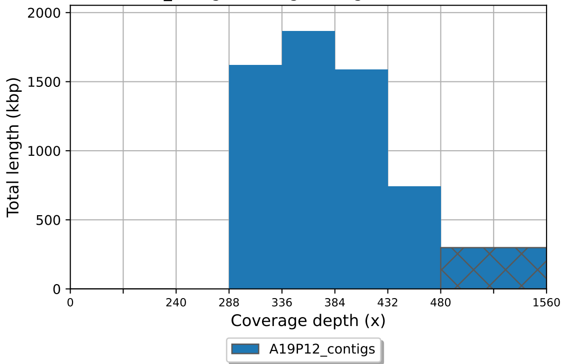
A19P12_contigs coverage histogram (bin size: 48x)
