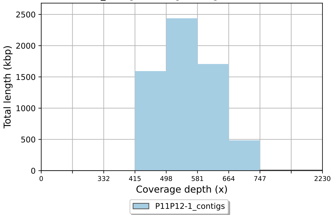
P11P12-1_contigs coverage histogram (bin size: 83x)
