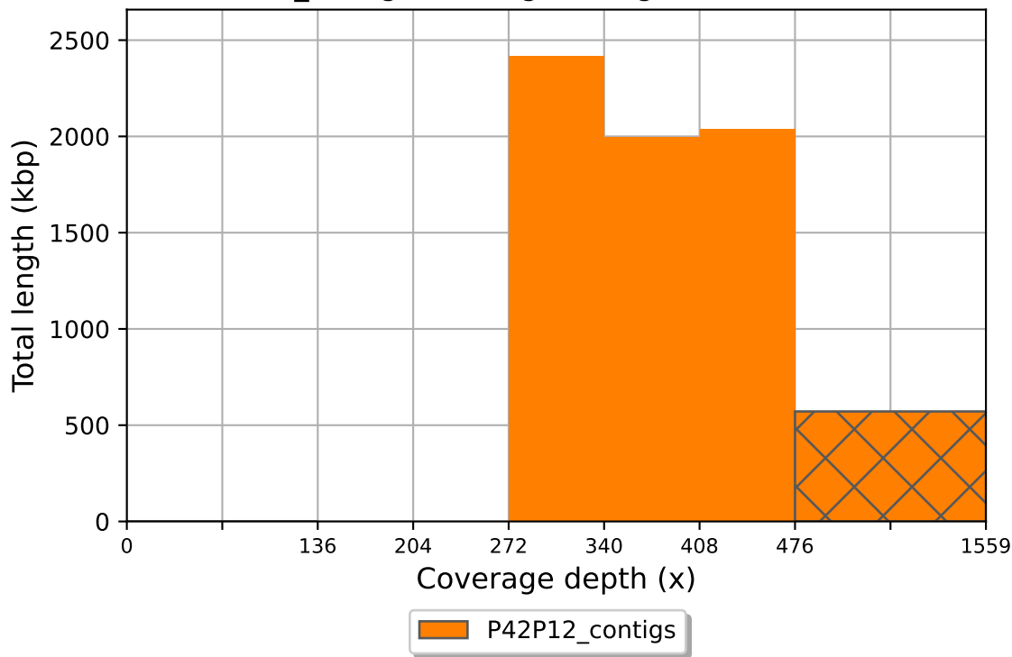
P42P12_contigs coverage histogram (bin size: 68x)
