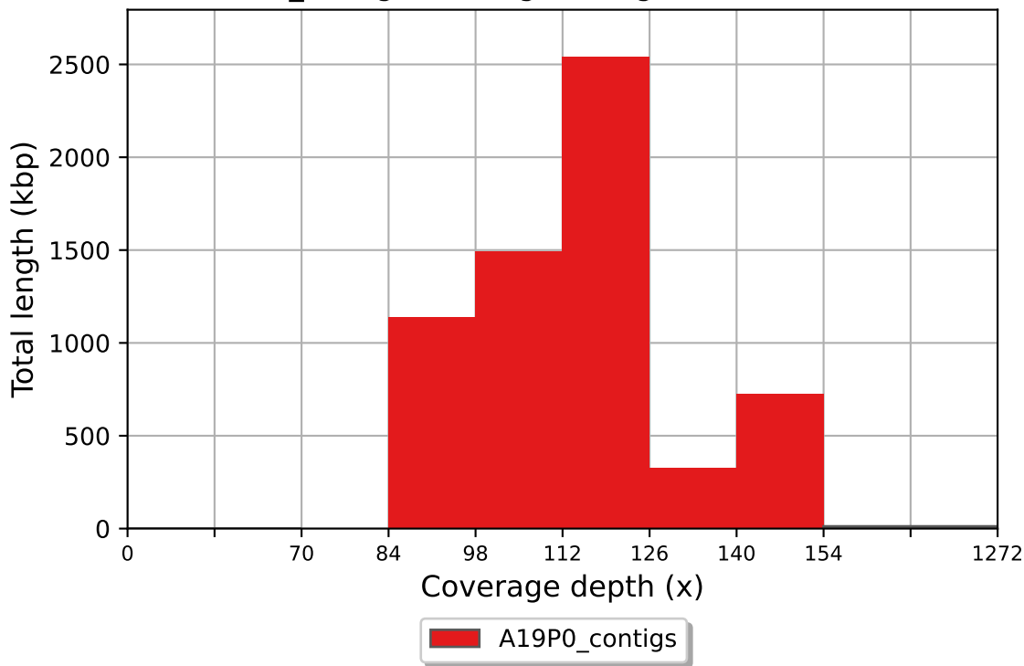
A19P0_contigs coverage histogram (bin size: 14x)
