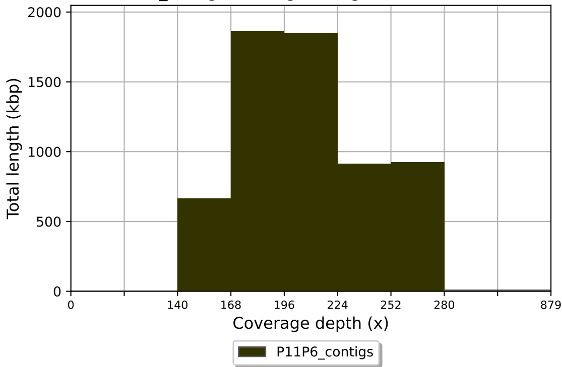
P11P6_contigs coverage histogram (bin size: 28x)
