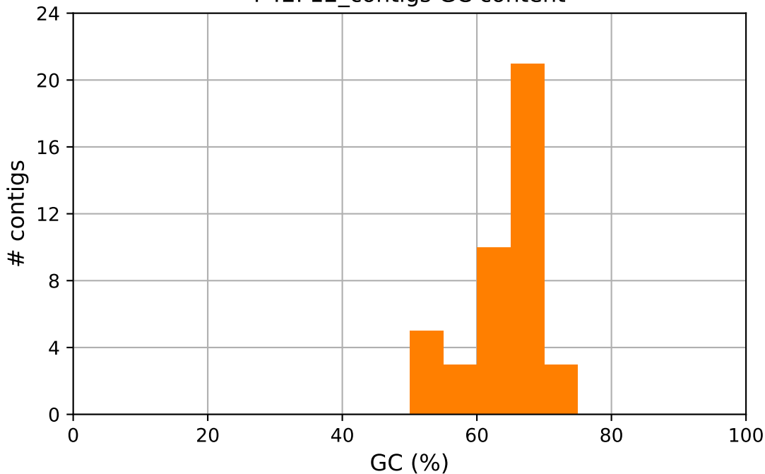
P42P12_contigs GC content
