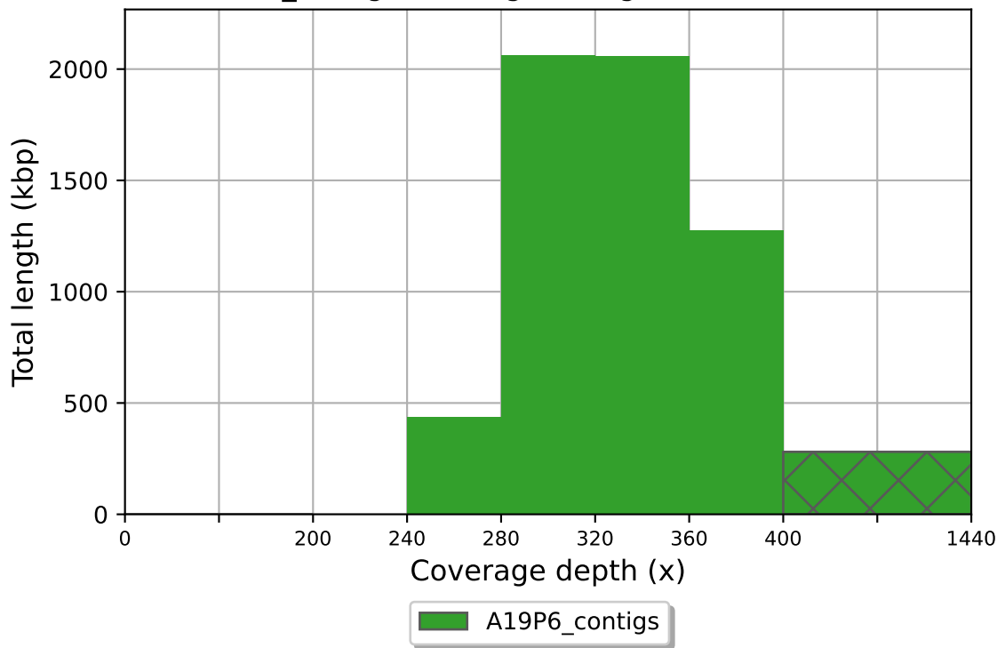
A19P6_contigs coverage histogram (bin size: 40x)
