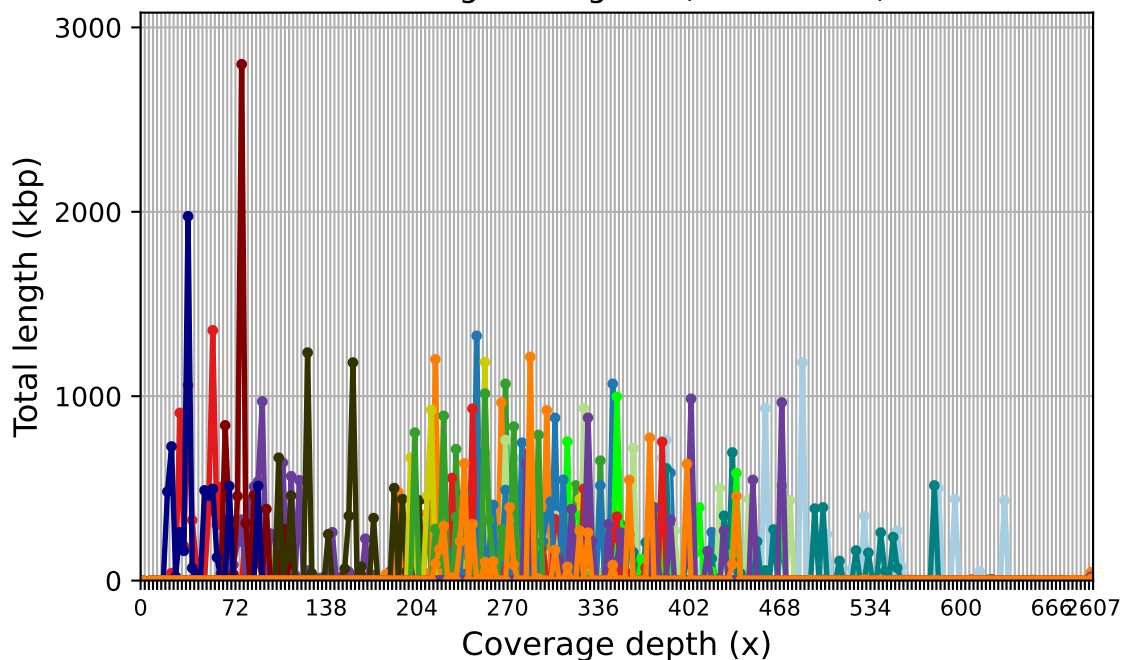
Coverage histogram (bin size: 3x)
