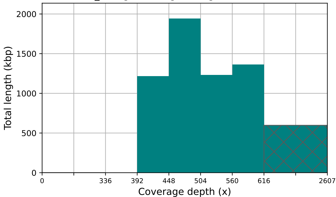
P3P12_contigs coverage histogram (bin size: 56x)
