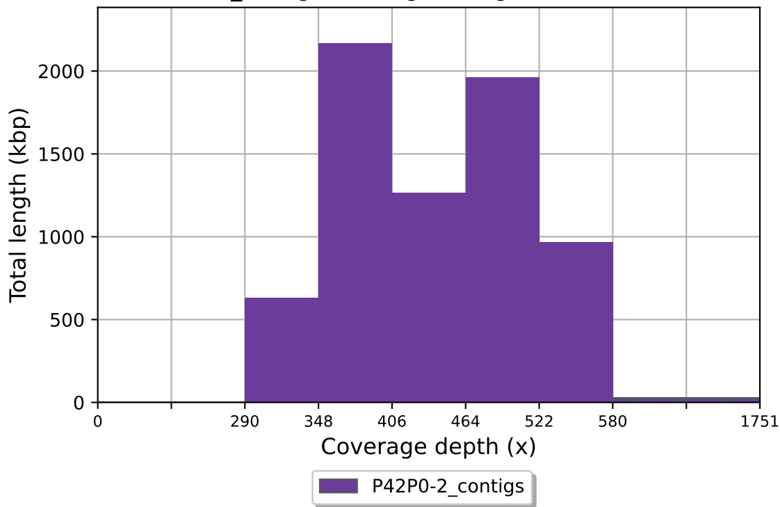
P42P0-2_contigs coverage histogram (bin size: 58x)
