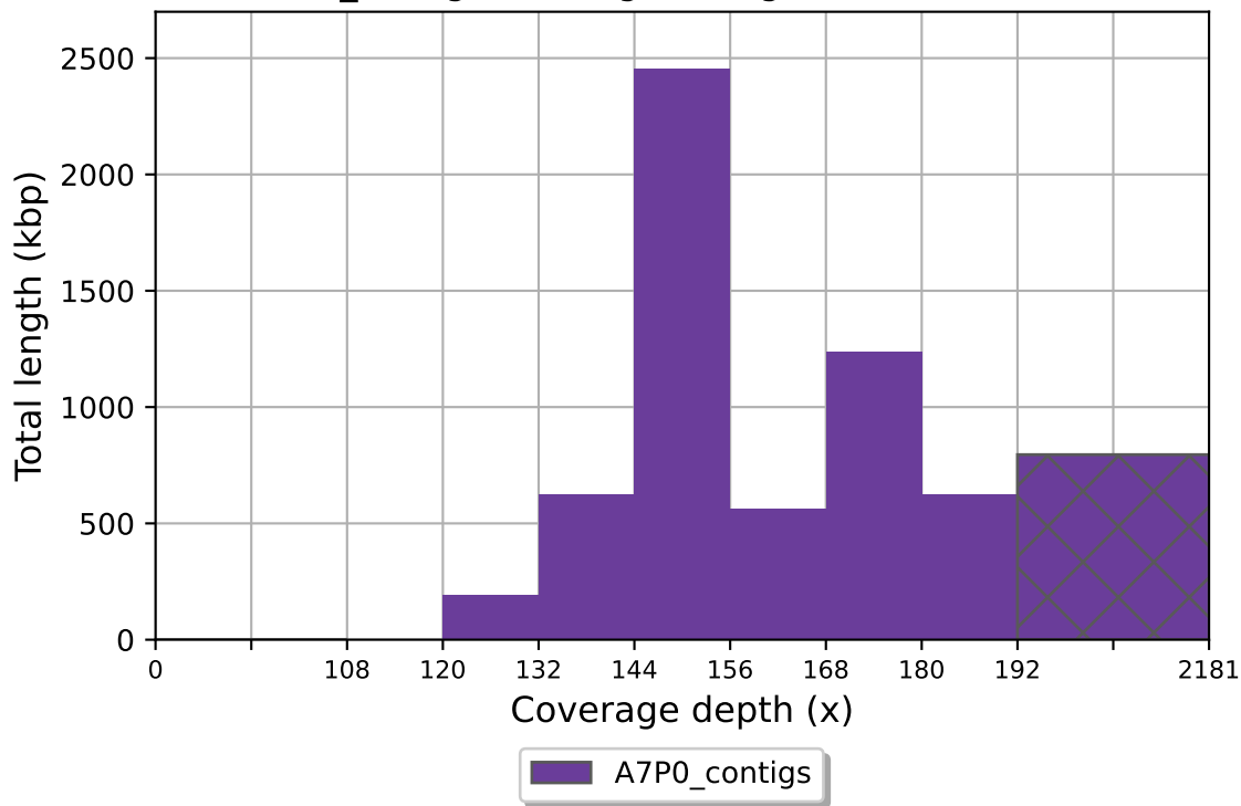
A7P0_contigs coverage histogram (bin size: 12x)
