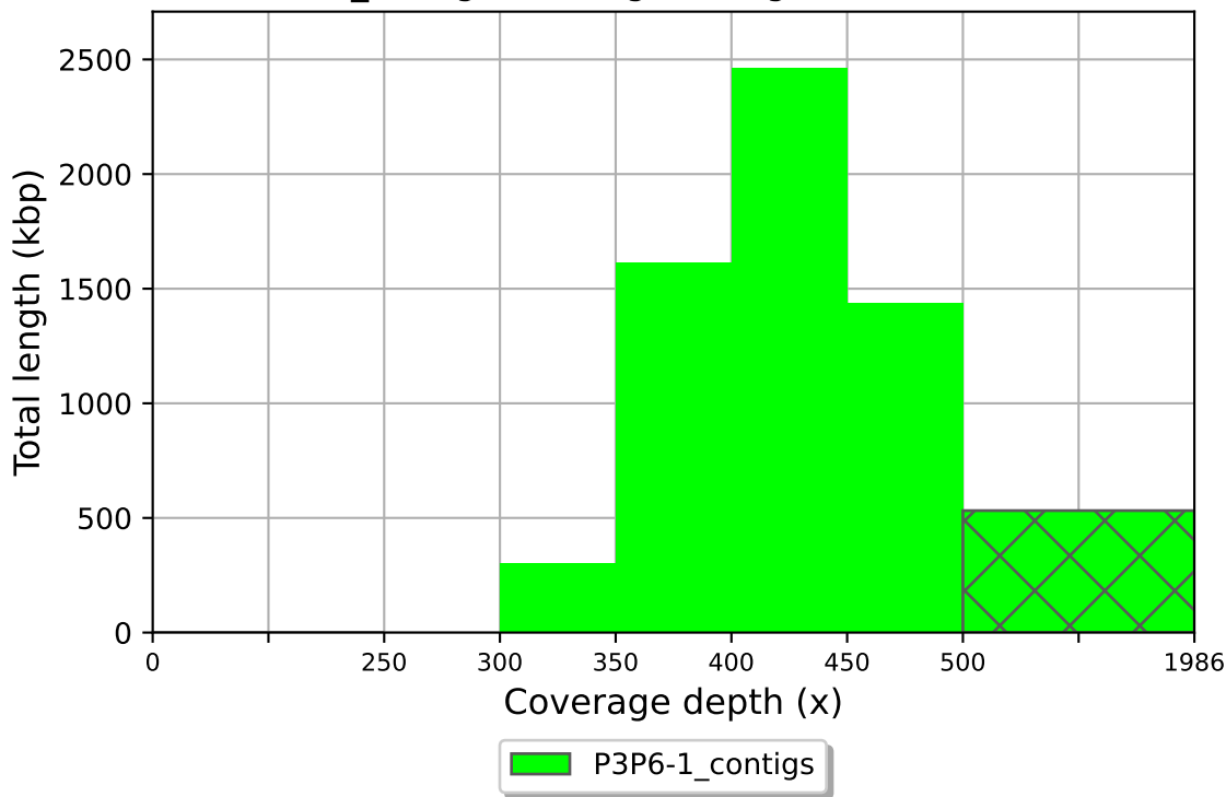
P3P6-1_contigs coverage histogram (bin size: 50x)
