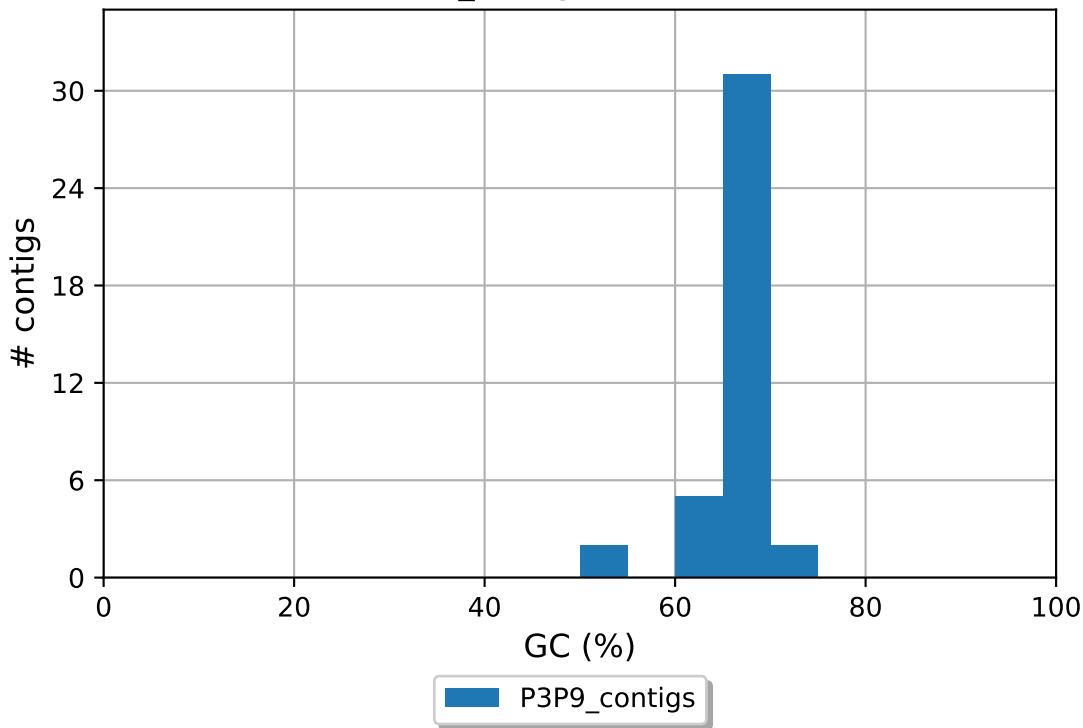
P3P9_contigs GC content
