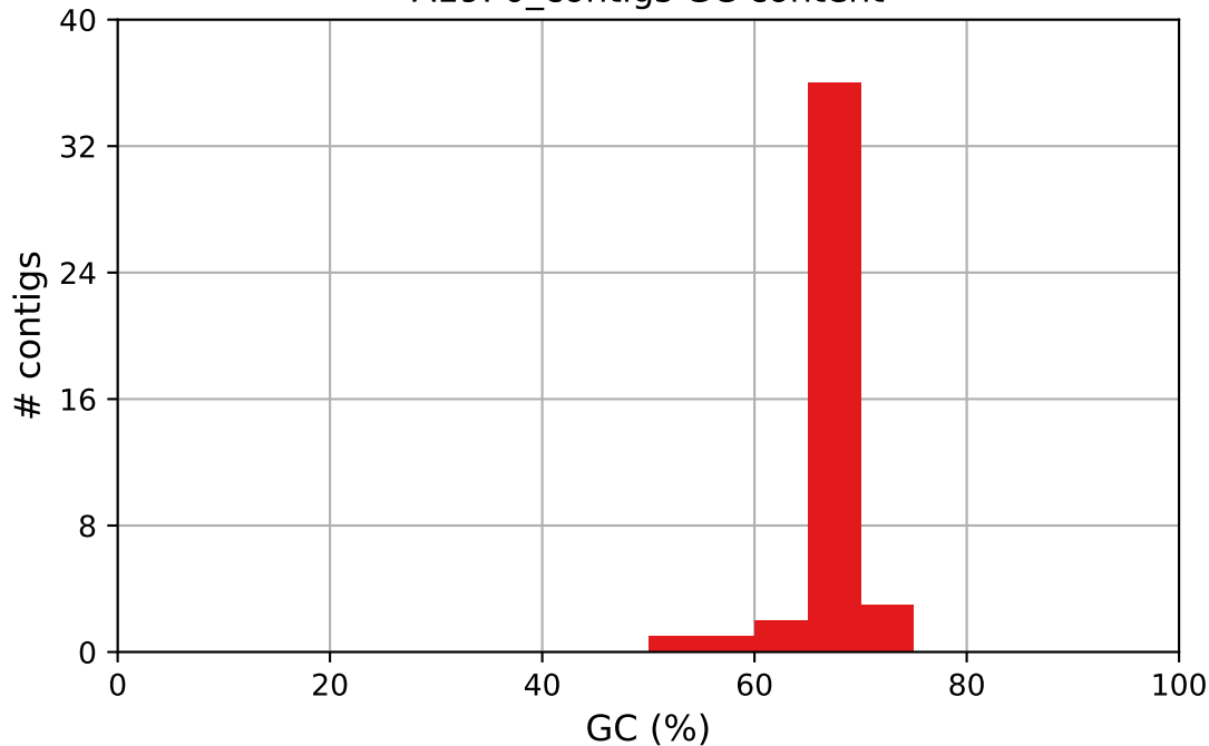
A19P0_contigs GC content
