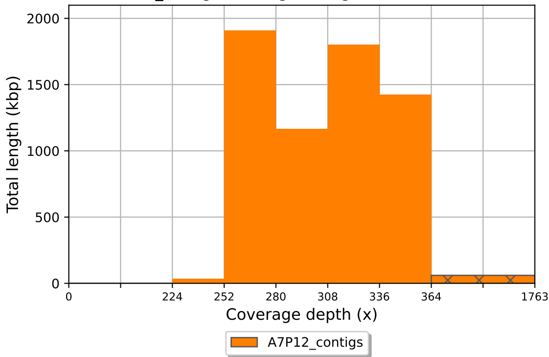
A7P12_contigs coverage histogram (bin size: 28x)
