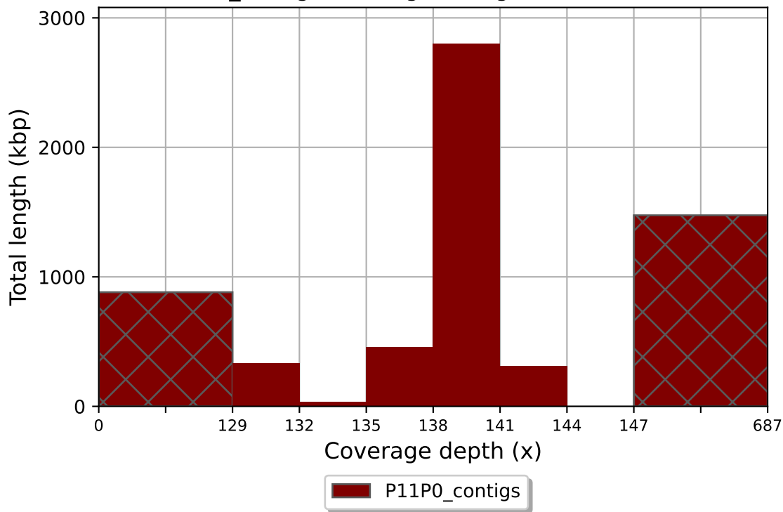
P11P0_contigs coverage histogram (bin size: 3x)
