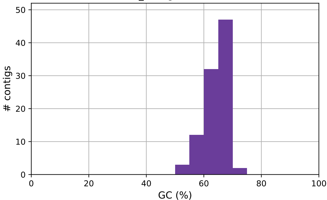
A7P0_contigs GC content
