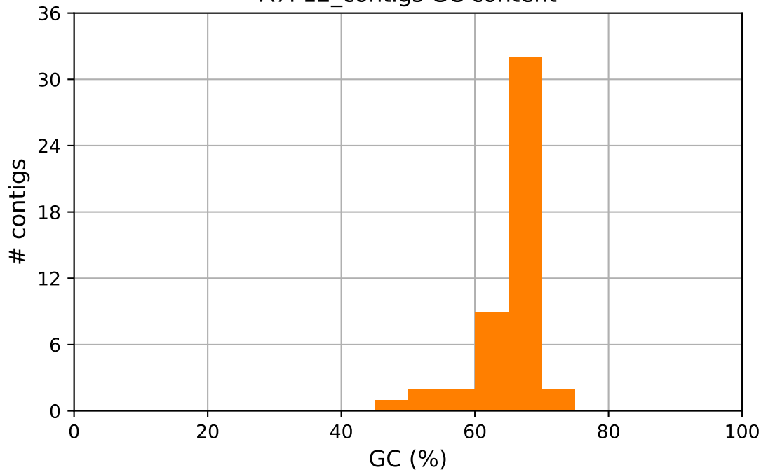
A7P12_contigs GC content
