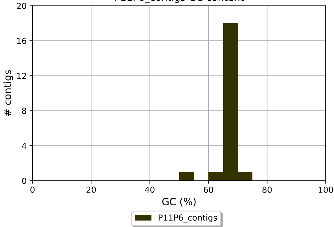
P11P6_contigs GC content
