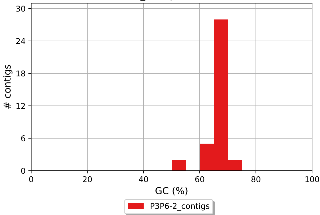
P3P6-2_contigs GC content
