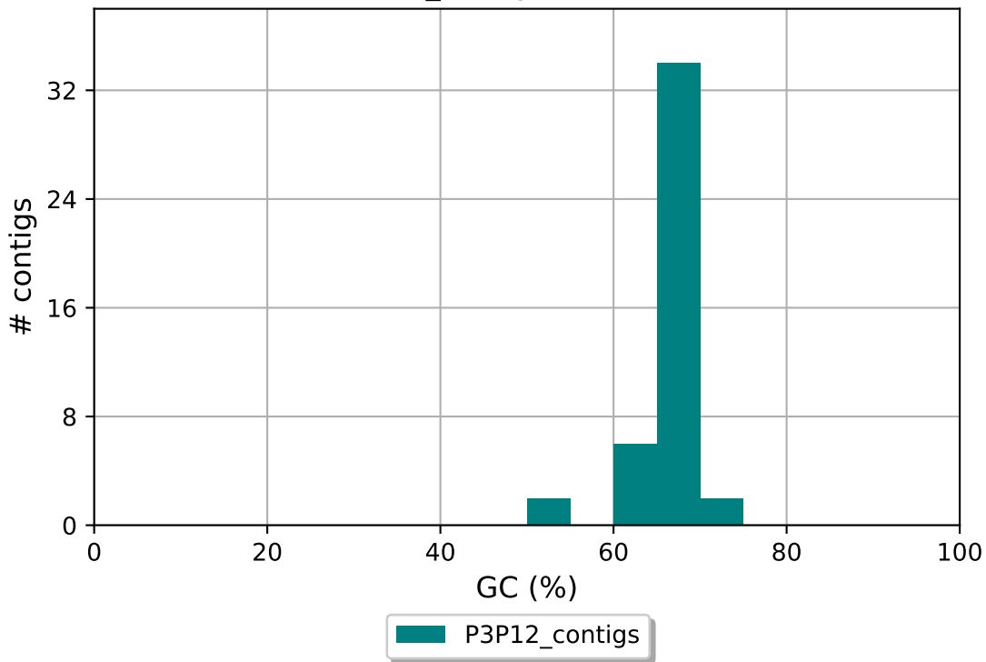
P3P12_contigs GC content
