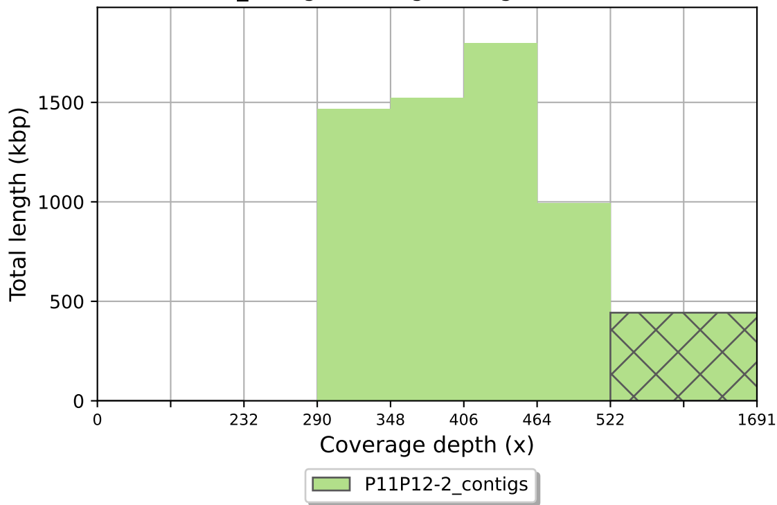
P11P12-2_contigs coverage histogram (bin size: 58x)
