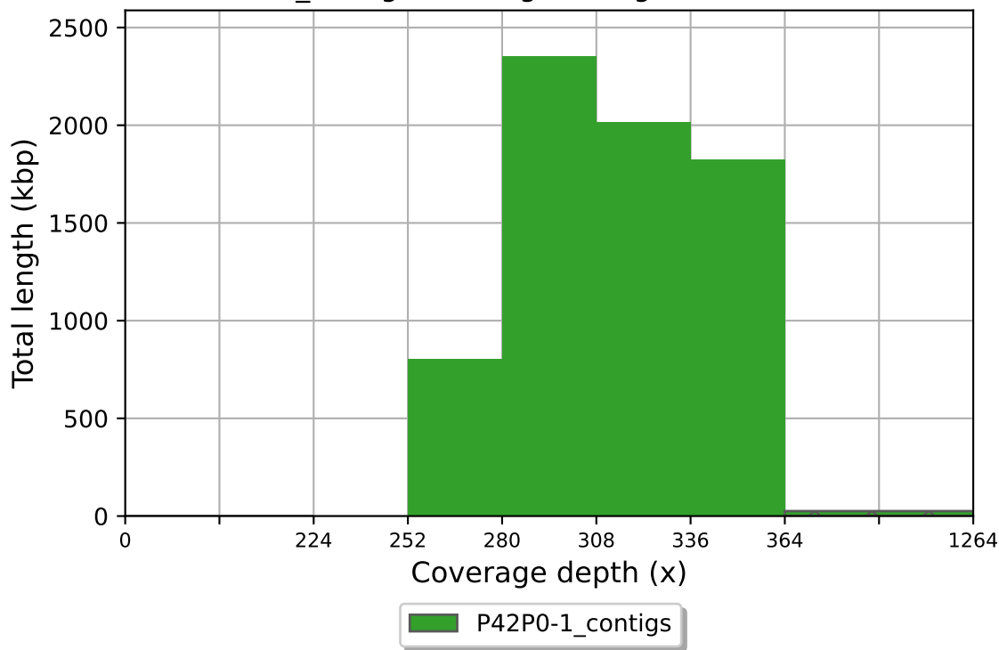
P42P0-1_contigs coverage histogram (bin size: 28x)
