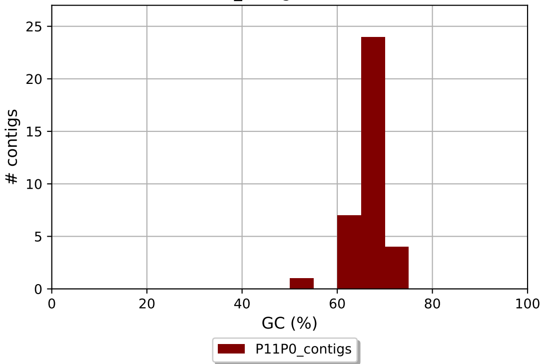
P11P0_contigs GC content
