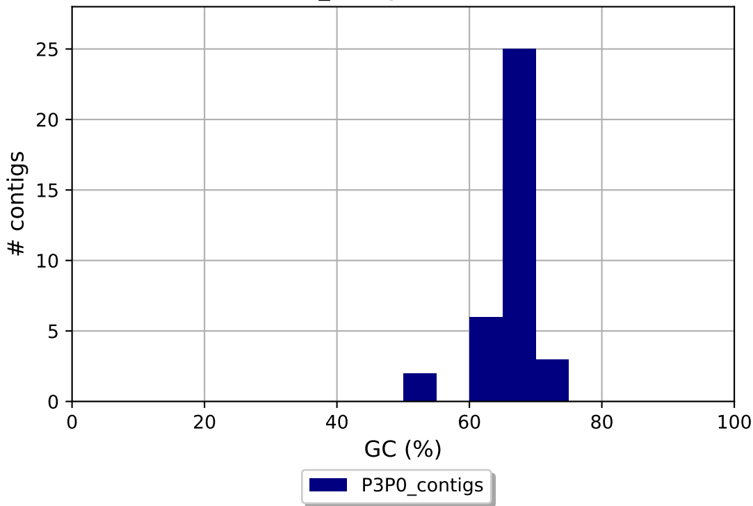
P3P0_contigs GC content
