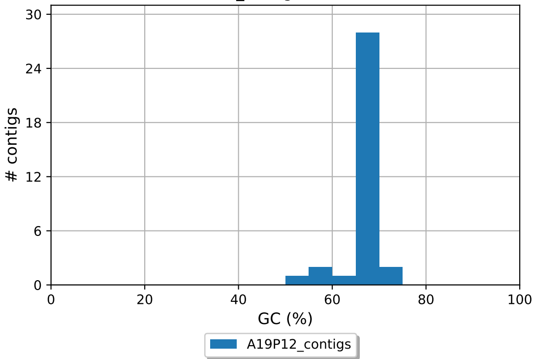
A19P12_contigs GC content
