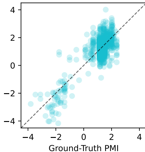
KDE MSE=2.040 (Raw)
