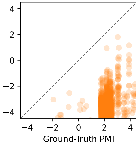
MINE MSE=35.340 (Raw)
