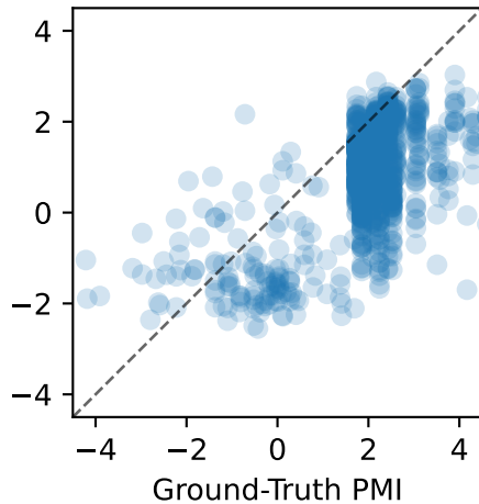
PMIScore MSE=2.363 (Raw)
