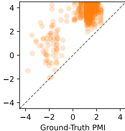
MINE MSE=7.080 (Raw)
