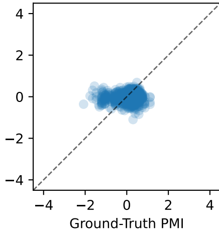
PMIScore MSE=0.266 (Raw)
