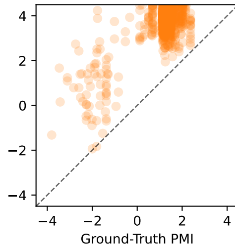
MEEP MSE=1.609 (Scaled)
