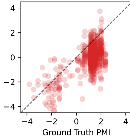
KDE MSE=2.040 (Raw)
