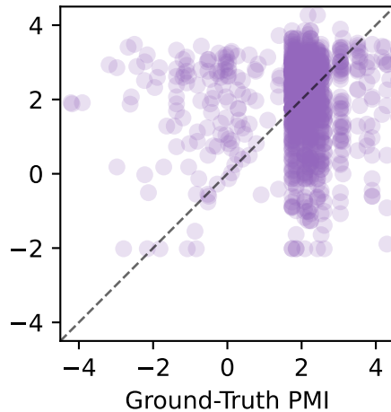
MEEP MSE=2.927 (Scaled)
