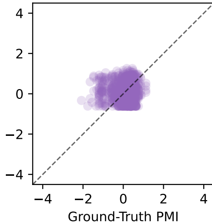
MEEP MSE=0.401 (Scaled)
