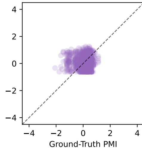
MEEP MSE=0.401 (Scaled)
