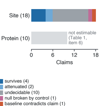
c Verdicts
